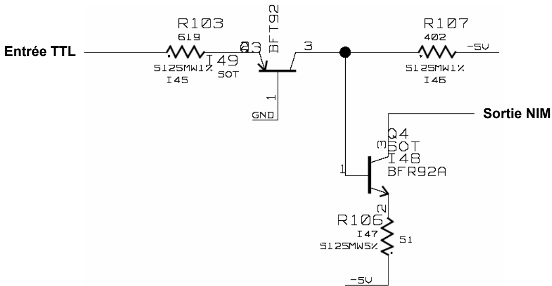
Figure 20 : Conversion TTL→NIM
