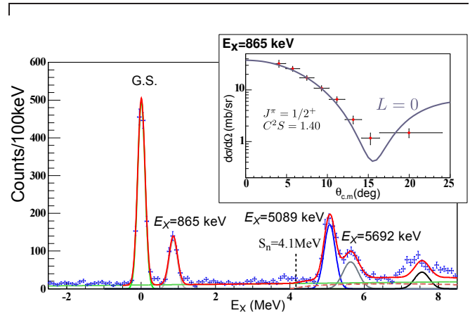
FIG. 2. (color online). Experimental missing mass spectrum for the ^{16}\text{O}(d,p)^{17}\text{O} reaction in inverse kinematics. Dashed line (brown): 3-body phase space. Thin solid line (green): background from reactions of the beam with the carbon of the \text{CD}_2 target. Inset: sample angular distribution for the first excited state, compared to a DWBA calculation.
