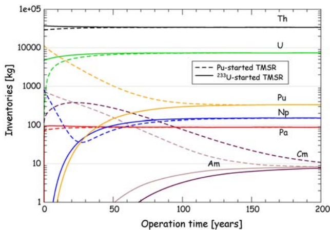
Fig.14. Heavy nuclei inventory for the 233 U-started TMSR (solid lines) and for the Pu-started TMSR (dashed lines)
