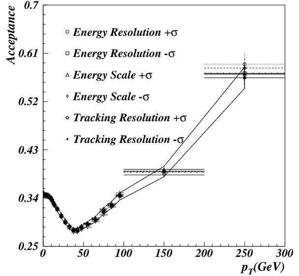
FIG. 11. Effect of uncertainties on the acceptance in each bin of p_T . The band corresponds to a parameterization of the uncertainty as a function of p_T , as discussed in the text.
