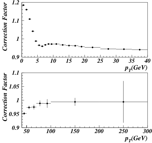
FIG. 21. Smearing correction factor \alpha(p_T) as a function of p_T .
