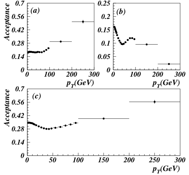
FIG. 10. Final acceptance as a function of p_T for (a) the CCC, (b) CCEC event topologies, and (c) for the combined event sample.
