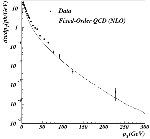
FIG. 26. Plot of the differential cross section (circles) as a function of p_T . The line is the result of the fixed-order (NLO) calculation of the differential cross section.
