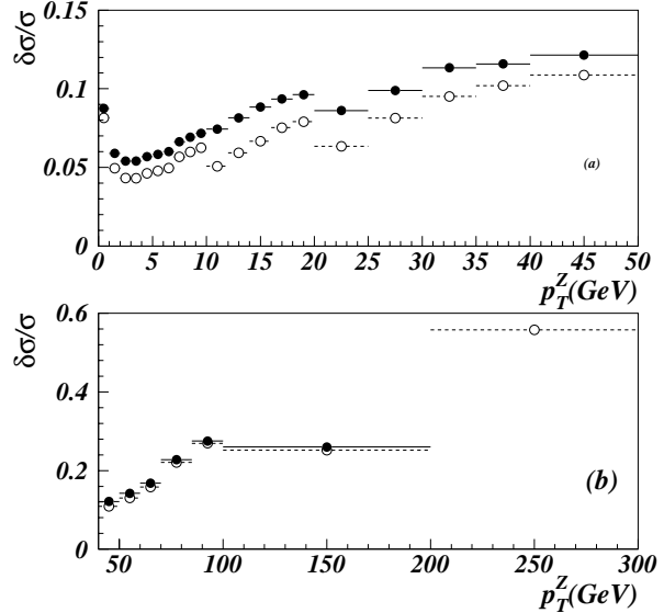
FIG. 22. Fractional uncertainty in the cross section as a function of p_T including the statistical and systematic uncertainties (closed circles) and including only statistical uncertainties (open circles) for (a) p_T < 50 \text{ GeV} and (b) p_T > 50 \text{ GeV} .
