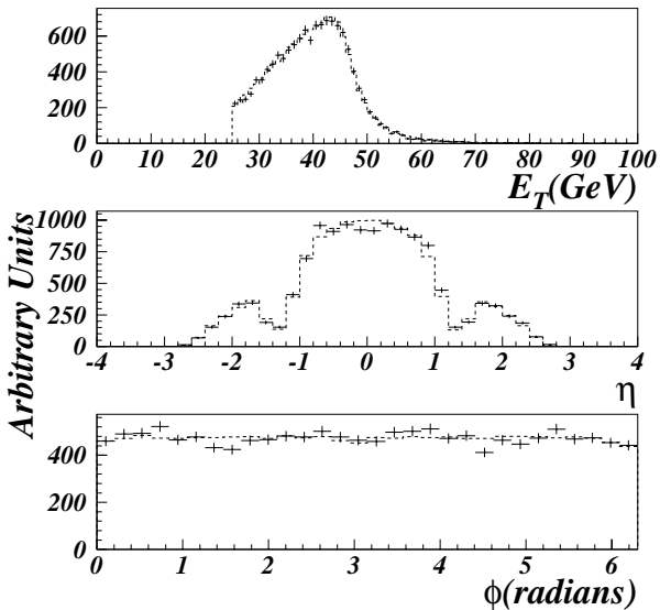
FIG. 4. Comparison of electron E_T , \eta , and \phi , from Z boson data (crosses) to results of the detector simulation (dashed).
