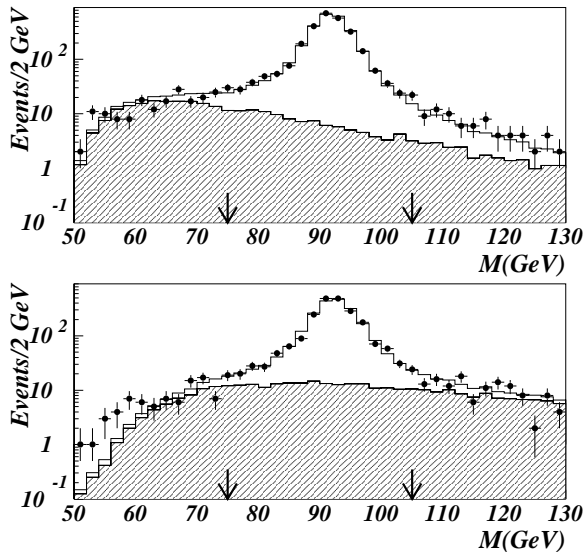
FIG. 17. Comparison of the dielectron invariant mass distribution (closed circles) and the background (dashed line) to the fit to PYTHIA Z/\gamma^* and background (solid line) for (a) CCCC and (b) CCEC topologies.
