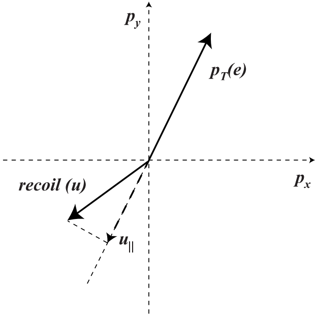
FIG. 5. Illustration of the relationship between the transverse momentum of the electron, the vector E_T of the hadron recoil ( u ) in the calorimeter, and u_{||} , the projection of the recoil onto the transverse direction of the electron. In the particular example illustrated here, u_{||} is negative.
