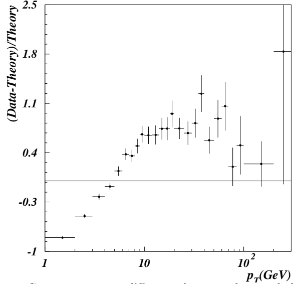
FIG. 28. Fractional difference between data and the fixed-order calculation from RESBOS for the differential cross section as a function of p_T .
