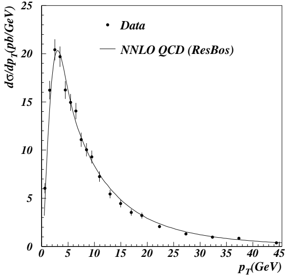
FIG. 23. Plot of the differential cross section (circles) as a function of p_T . The line is the result of the NNLO calculation from RESBOS using the CTEQ4M pdf. Theory has been normalized to the data.
