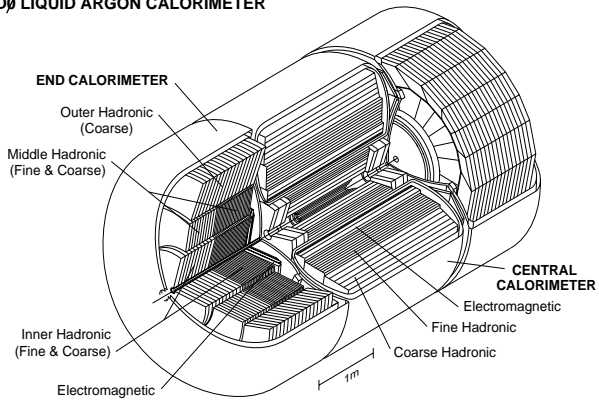
FIG. 1. A cutaway view of the DØ calorimeter and tracking system.
