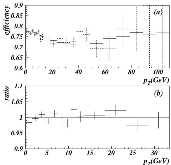
FIG. 6. (a) Comparison of the Z boson selection efficiency as a function of p_T as determined using HERWIG (dashed crosses), and as determined using a parameterization of the single-electron efficiency as a function of u_{||} (solid crosses). (b) The ratio of the two methods in the range 0–30 GeV, where they are expected to agree.
