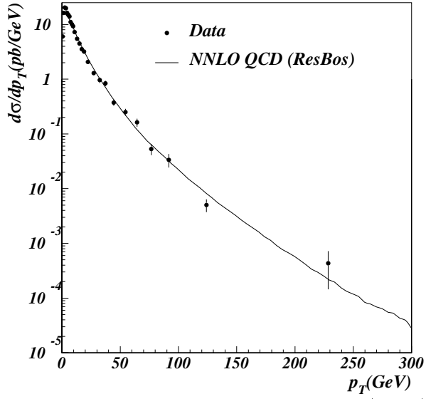
FIG. 25. Plot of the differential cross section (circles) as a function of p_T . The line is from the NNLO calculation from RESBOS using CTEQ4M as the pdf. Theory has been normalized to the data.
