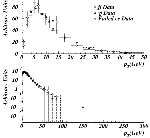
FIG. 15. Comparison of shapes of transverse momentum distributions for the three multijet background samples for the CCEC event topology.
