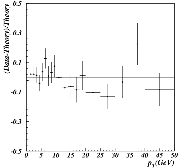
FIG. 24. Fractional difference between the data and the NNLO calculation from RESBOS for the differential cross section as a function of p_T .
