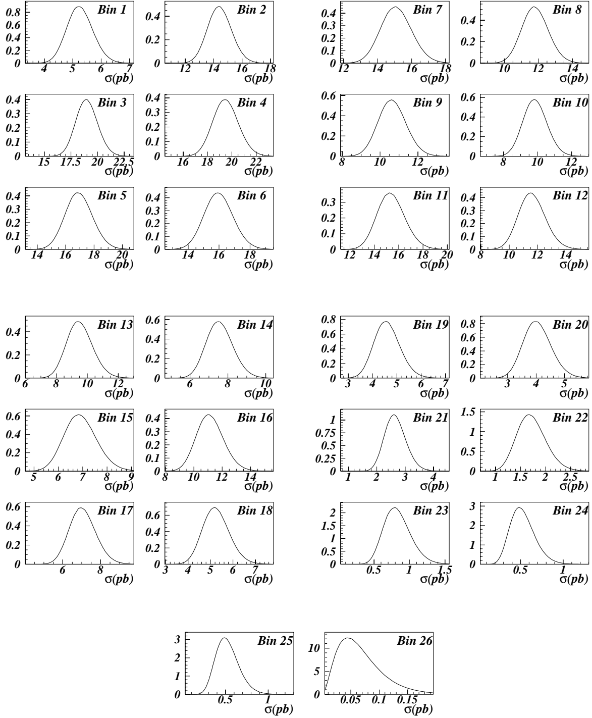
FIG. 20. Normalized probability distributions for cross sections ( \sigma ) in individual bins of p_T . The vertical scale in each case is Probability/pb.
