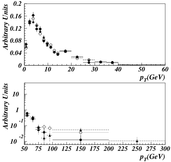
FIG. 9. Comparison of the transverse momentum distribution of dielectron pairs with mass very close to the nominal Z boson mass, 90 < M_{ee} < 92 GeV (solid circles) to those in the mass regions 75 < M_{ee} < 90 GeV (open circles) and 92 < M_{ee} < 105 GeV (closed triangles).
