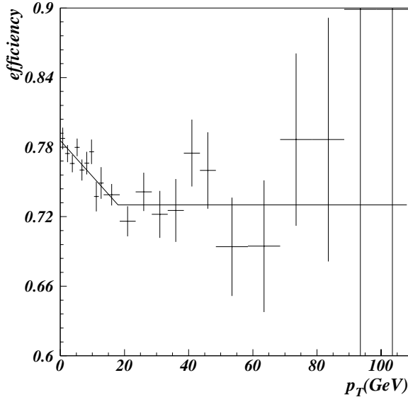
FIG. 7. Final event identification efficiency as a function of p_T , based on HERWIG events; the line is the parameterization used in calculating the final cross section.
