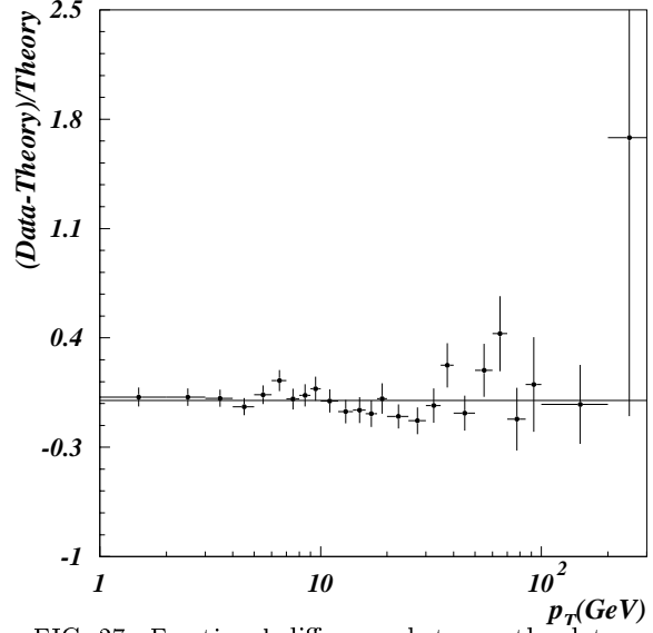
FIG. 27. Fractional difference between the data and the NNLO calculation from RESBOS for the differential cross section as a function of p_T .
