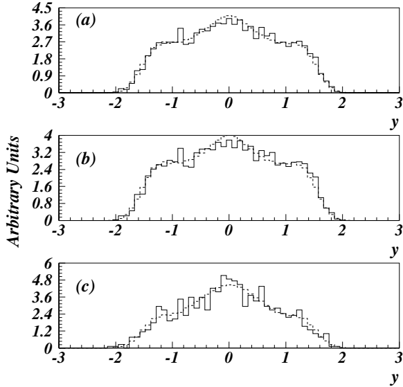
FIG. 12. Comparison of Z boson rapidity ( y ) distribution for the data (solid) and the simulation (dashed) for (a) all values of p_T , (b) p_T < 20 GeV, and (c) 20 < p_T < 50 GeV.
