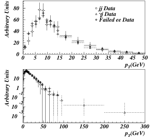
FIG. 16. Comparison of shapes of transverse momentum distributions for the three multijet background samples for the CCCC event topology.
