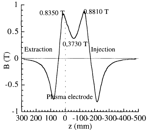
Figure 4: axial magnetic profile of the nanogan 2 ion source.
