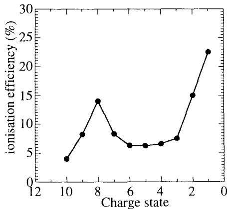
Figure 7: Ionisation efficiency of stable ^{40}\text{Ar} on the different charge states.
