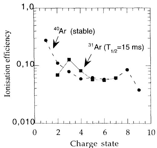
Figure 8: Comparison of ^{31}\text{Ar} charge state distribution with the ^{40}\text{Ar} distribution.
