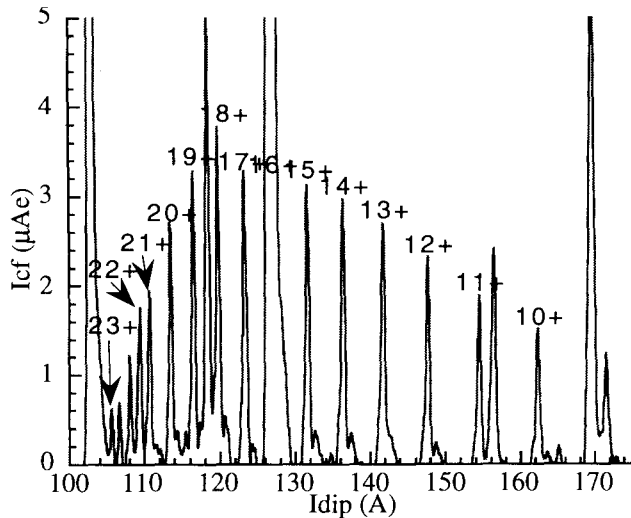
Figure 6: Charge state distribution of xenon when the source is optimised to produce \text{Xe}^{23+}
