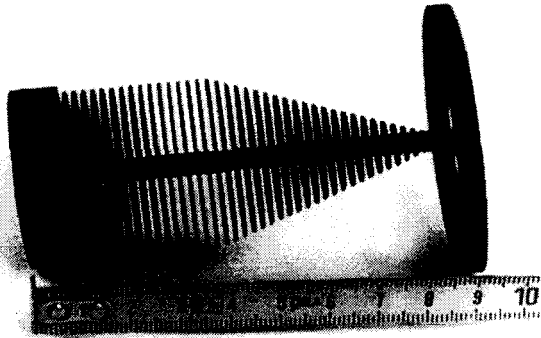
Figure 2: picture of the conical sliced target used during the Louvain la Neuve tests.
