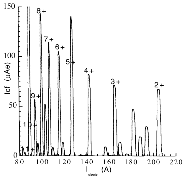
Figure 5: Charge state distribution of argon when the source is optimised to produce Ar^{8+}
