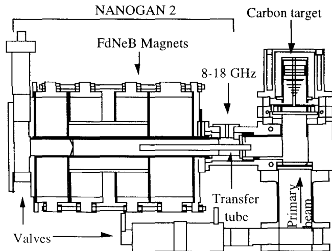
Figure 3: Schematic drawing of the first target ion source system for the spiral project.
