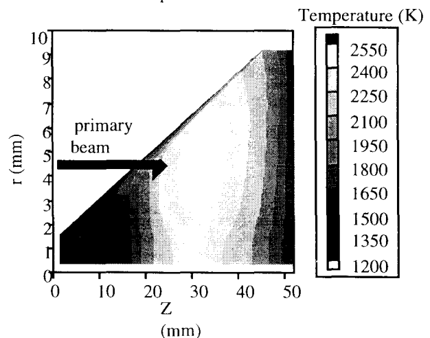
Figure 1: temperature distribution of a carbon target heated by a 2 kW Argon primary beam.
