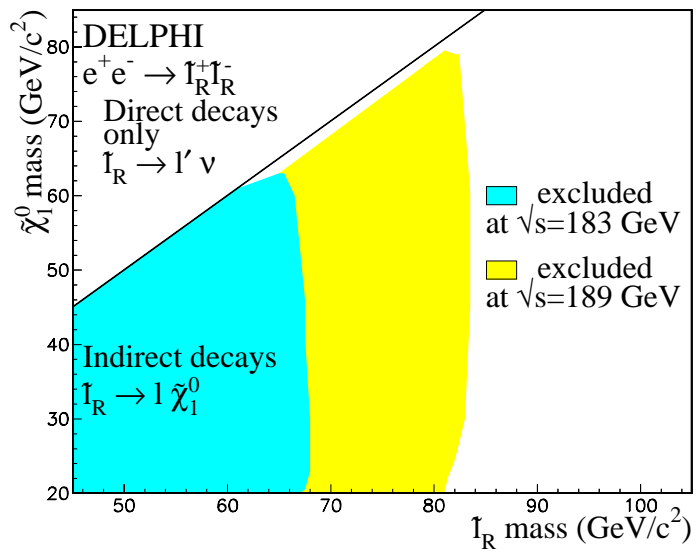
Figure 6: Charged slepton indirect decay: excluded region at 95% C.L. in m_{\tilde{\chi}^0} , m_{\tilde{\ell}_R} parameter space by \tilde{\ell}_R pair production. The dark grey area shows the part excluded by the searches at 183 GeV, the light grey area the one excluded by the present searches at 189 GeV.
