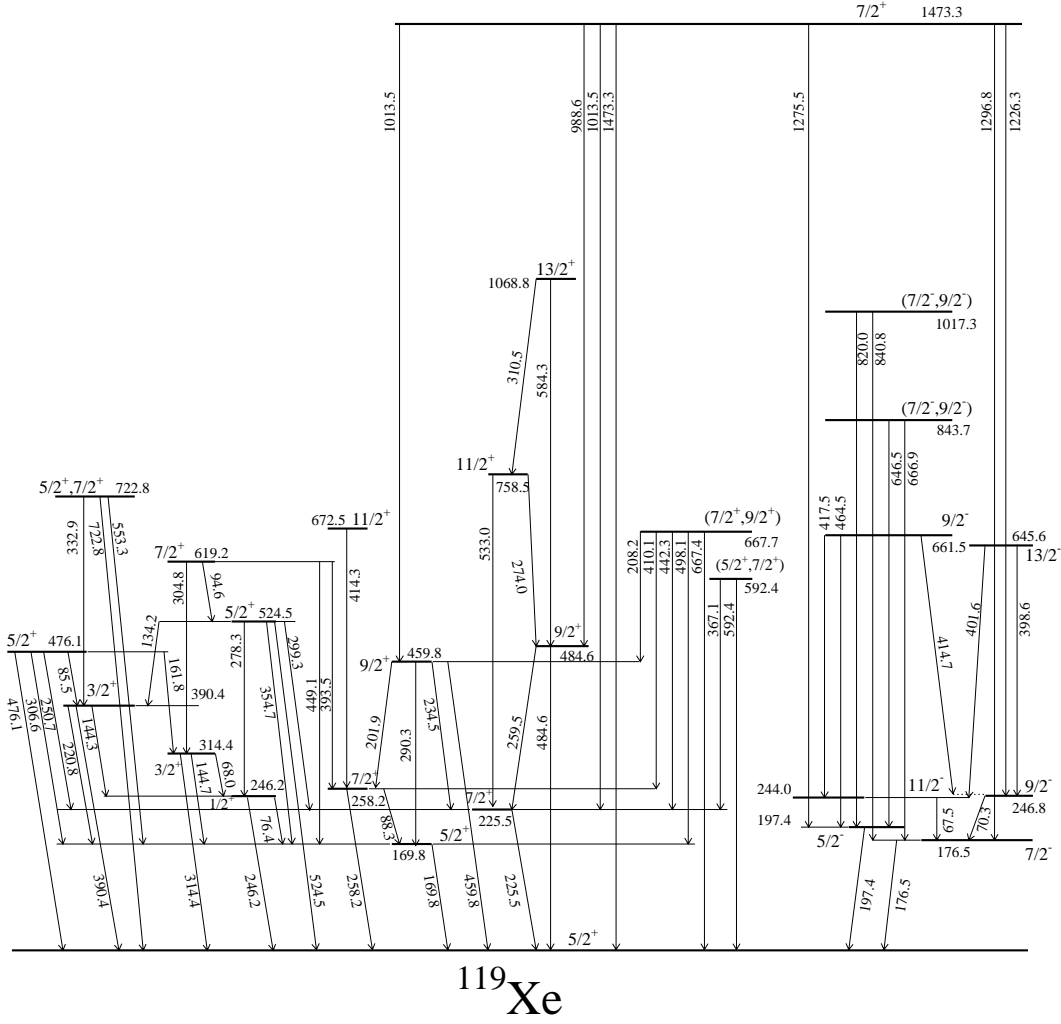
Figure 7: Low-energy part of the ^{119}\text{Xe} level scheme obtained in the ^{119m.g}\text{Cs} decay, showing the first members of band structures and their connexions. Transition and level energies are given in keV.
