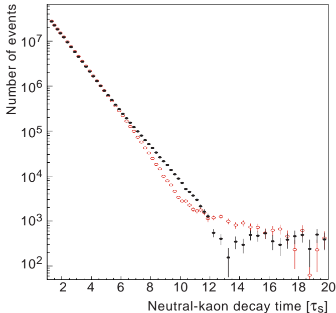
Figure 16: The measured decay rates for K^0 (open circles) and \bar{K}^0 (solid circles) after acceptance correction and background subtraction.
