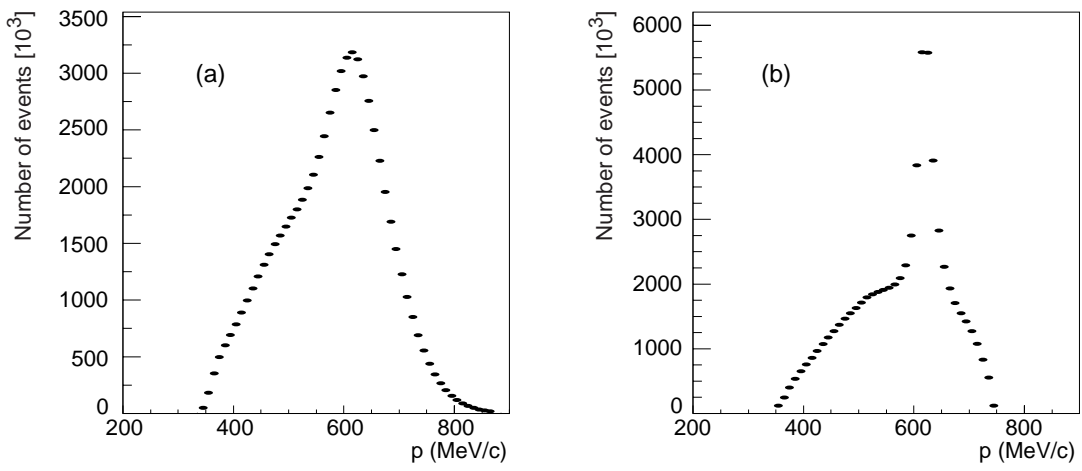
Figure 8: Charged kaon momentum distribution for data after (a), track fit, and (b), 9C fit.
