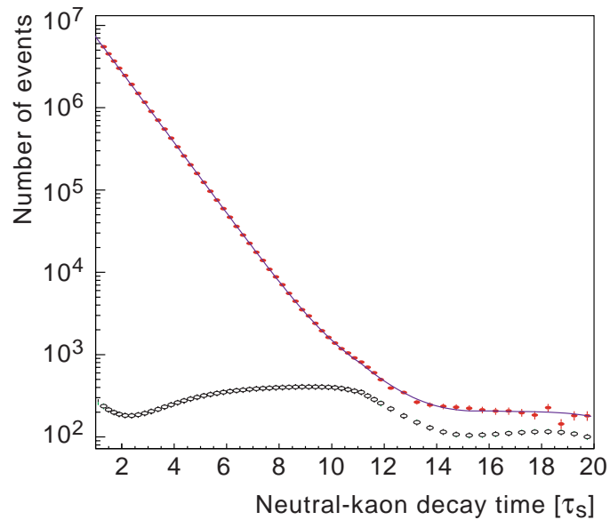
Figure 15: The measured decay rate (acceptance corrected) for K^0 plus \bar{K}^0 . The continuous curve is a fit to the data. The open circles show the calculated background level.
