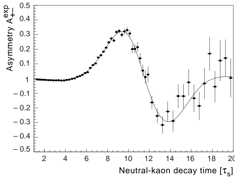
Figure 17: The measured decay rate asymmetry, A_{+-}^{\text{exp}}(\tau) . The solid circles are the data points, including residual background, while the continuous curve is the result of our fit.
