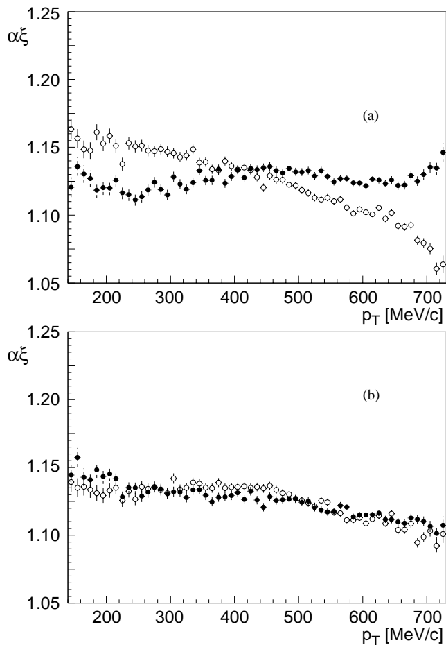
Figure 12: The dependence of \alpha\xi on the neutral-kaon transverse momentum p_T , when (a) K^0 and \bar{K}^0 events are measured with the same field polarity, positive (open circles) or negative (closed circles) (b) K^0 and \bar{K}^0 events are measured with opposite field polarities, so that the charged kaons have the same curvature sign, positive (open circles) or negative (closed circles).
