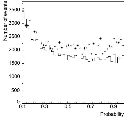
Figure 5: 1C fit probability distribution for data and Monte Carlo (●) above 10% probability.
