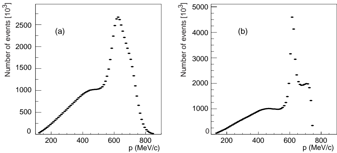
Figure 10: Neutral-kaon momentum distribution for data after (a), track fit, and (b), 9C fit.
