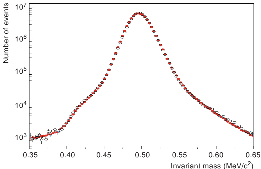
Figure 11: Invariant mass at the secondary vertex for real (closed circles) and simulated (open circles) data.
