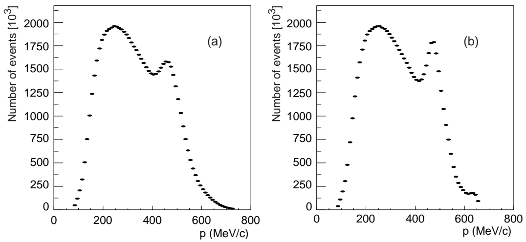
Figure 9: Primary pion momentum distribution for data after (a), track fit, and (b), 9C fit.
