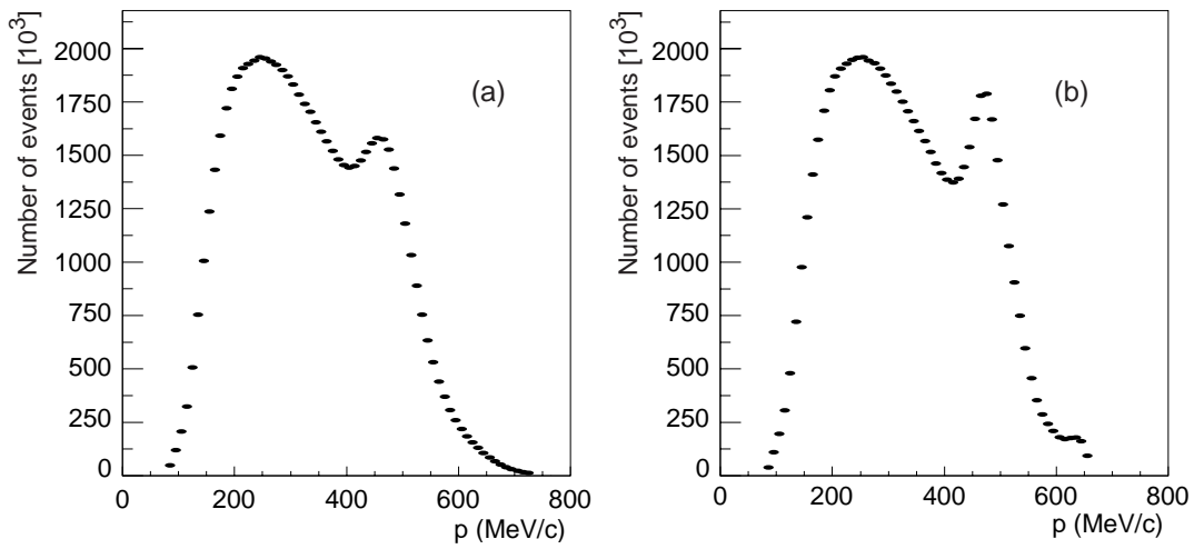
Figure 9: Primary pion momentum distribution for data after (a), track fit, and (b), 9C fit.
