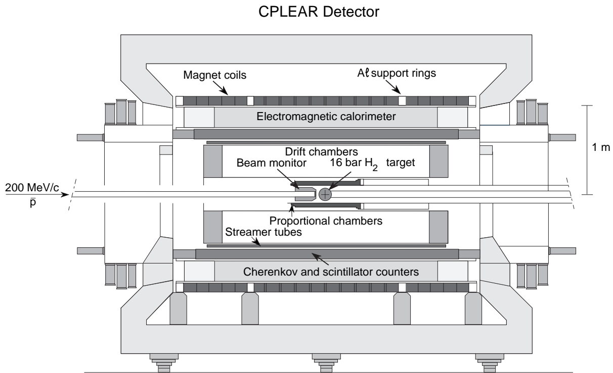
Figure 1: A longitudinal view of the CPLEAR detector prior to mid 1994.
