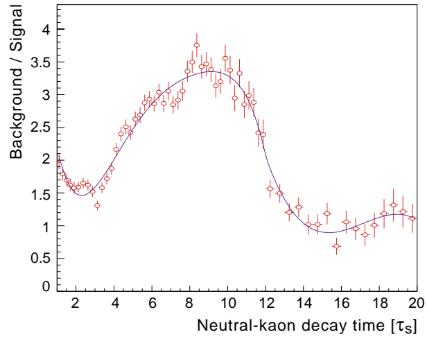
Figure 14: Ratio of K_L background to K_L signal ( K_L \rightarrow \pi^+\pi^- ). The continuous curve is a parametrised fit to the simulation data points.
