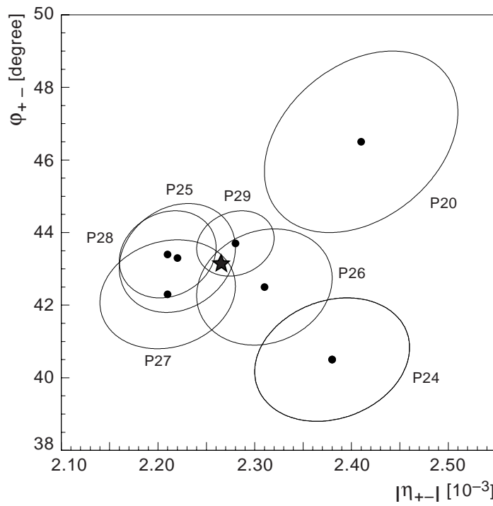
Figure 19: The one-sigma error ellipses for \phi_{+-} versus |\eta_{+-}| for each data-taking period (P20, P24-P29). The final result (★) is also shown.
