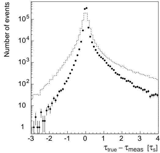
Figure 7: Difference between the true K^0 decay time and the measured decay time from the track fit and from the 9C constrained fit. (●)
