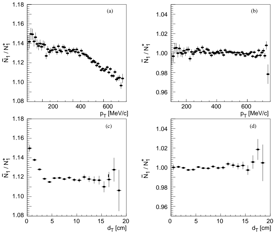
Figure 13: The ratios \overline{N}_1(p_T)/N_1^*(p_T) versus the neutral-kaon transverse momentum p_T (a) before and (b) after event weighting, and \overline{N}_1(d_T)/N_1^*(d_T) versus the vertex transverse separation d_T (c) before and (d) after event weighting. Note that the quantity displayed in (a) is in fact \alpha\xi(p_T) for data summed over the two field polarities.
