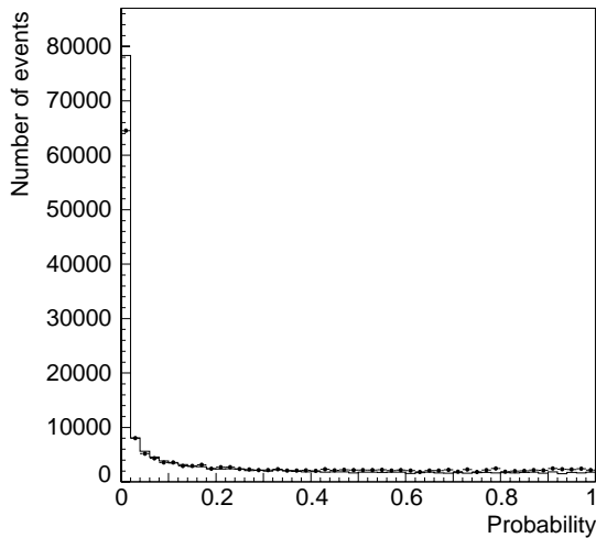
Figure 4: 1C fit probability distribution for data and Monte Carlo (●)
