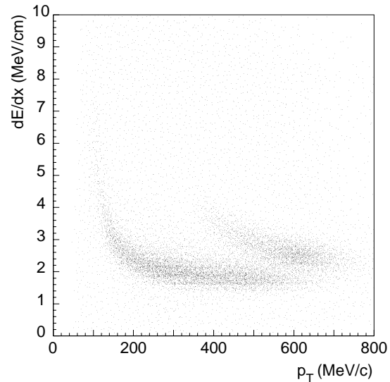
Figure 3: dE/dx vs p_T for all tracks in the event (Data).
