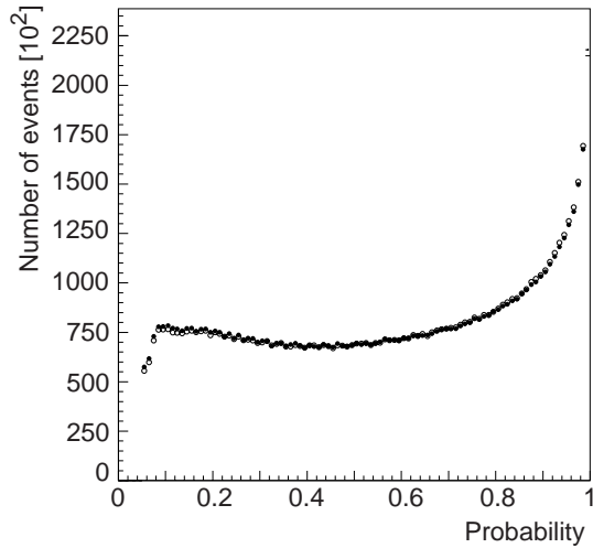
Figure 6: 9C fit probability distribution from real data for initial K^0 (closed circles) and \bar{K}^0 (open circles).
