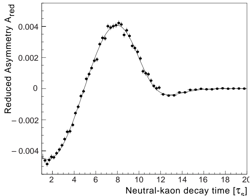
Figure 18: The ‘reduced asymmetry’ A_{\text{red}}(\tau) (see text) versus the neutral-kaon decay time. The continuous curve is the result of our fit.
