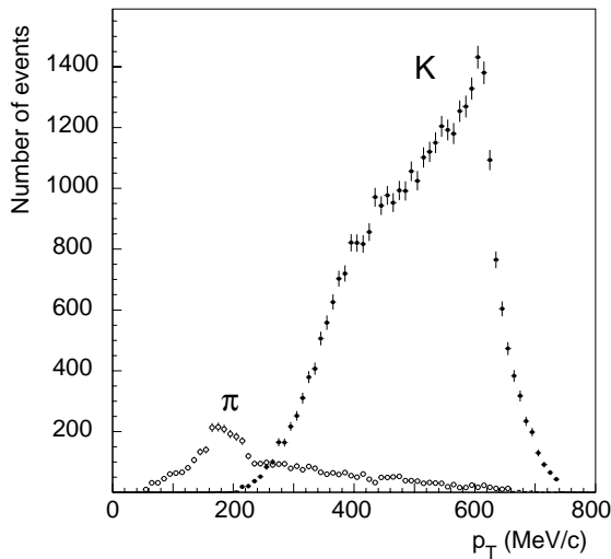
Figure 2: Tracks with an S\bar{C}S signature vs p_T (Monte Carlo).
