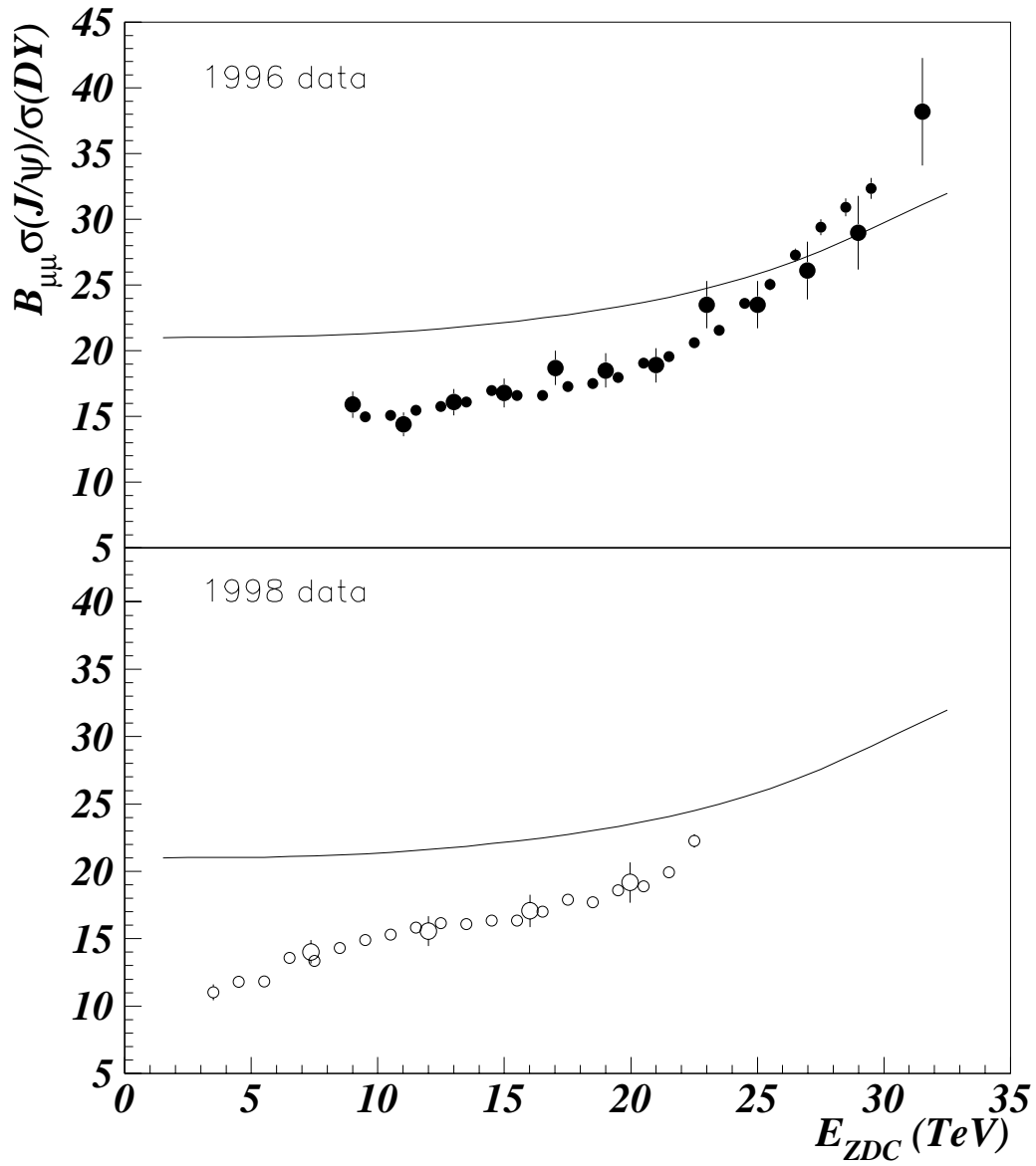
Figure 8: Comparison between the standard (large circles) and the minimum bias analysis (small circles) for the 1996 and 1998 data.
