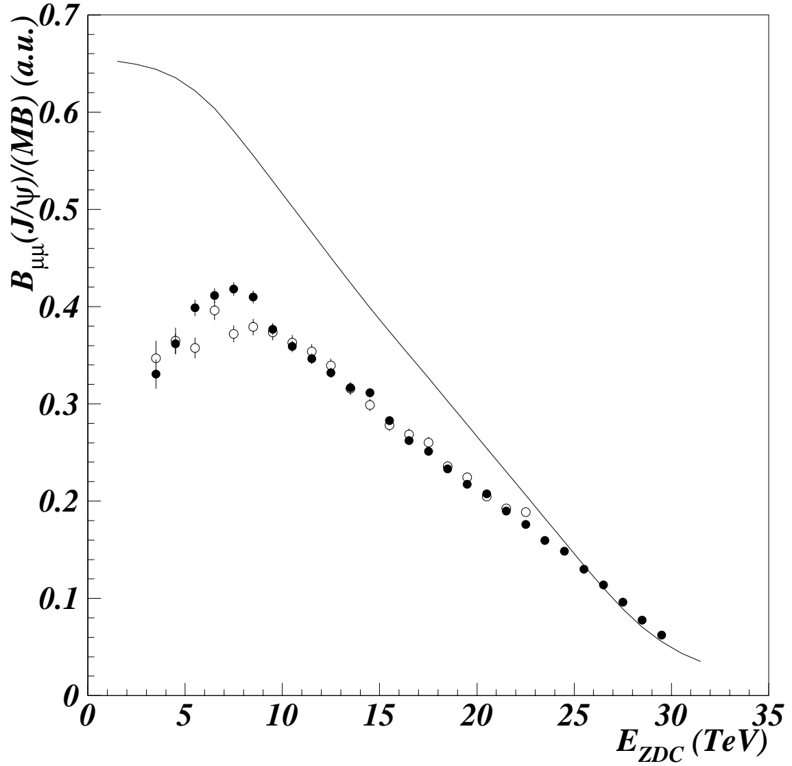
Figure 4: The ratio (J/\psi)/MB versus E_{ZDC} . Closed symbols correspond to 1996 data and open symbols to 1998 data. The curve represents the results of a Glauber calculation which takes into account the J/\psi suppression due to ordinary nuclear absorption, with \sigma_{J/\psi}^{abs} = 6.4 mb.
