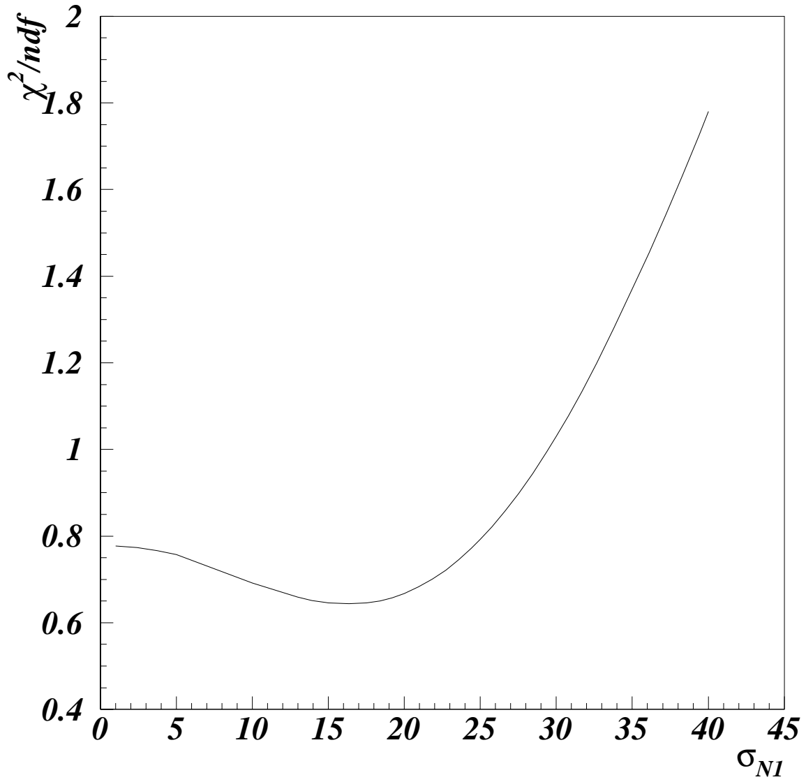
Figure 10: The quality of the fit of \sigma_{J/\psi}/\sigma_{DY^*} as a function of \sigma_{N1} (see text for details).
