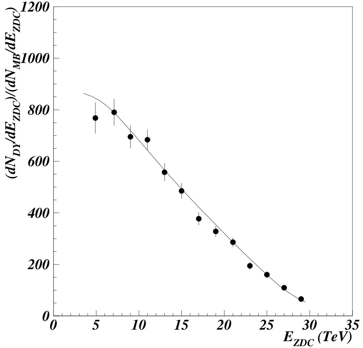
Figure 7: Comparison between the experimentally measured DY/MB ratio (closed circles) and the corresponding quantity in our calculation (continuous line). The Drell-Yan yield has been integrated in the interval 2.9 \leq M_{\mu\mu} \leq 4.5 \text{ GeV}/c^2 .
