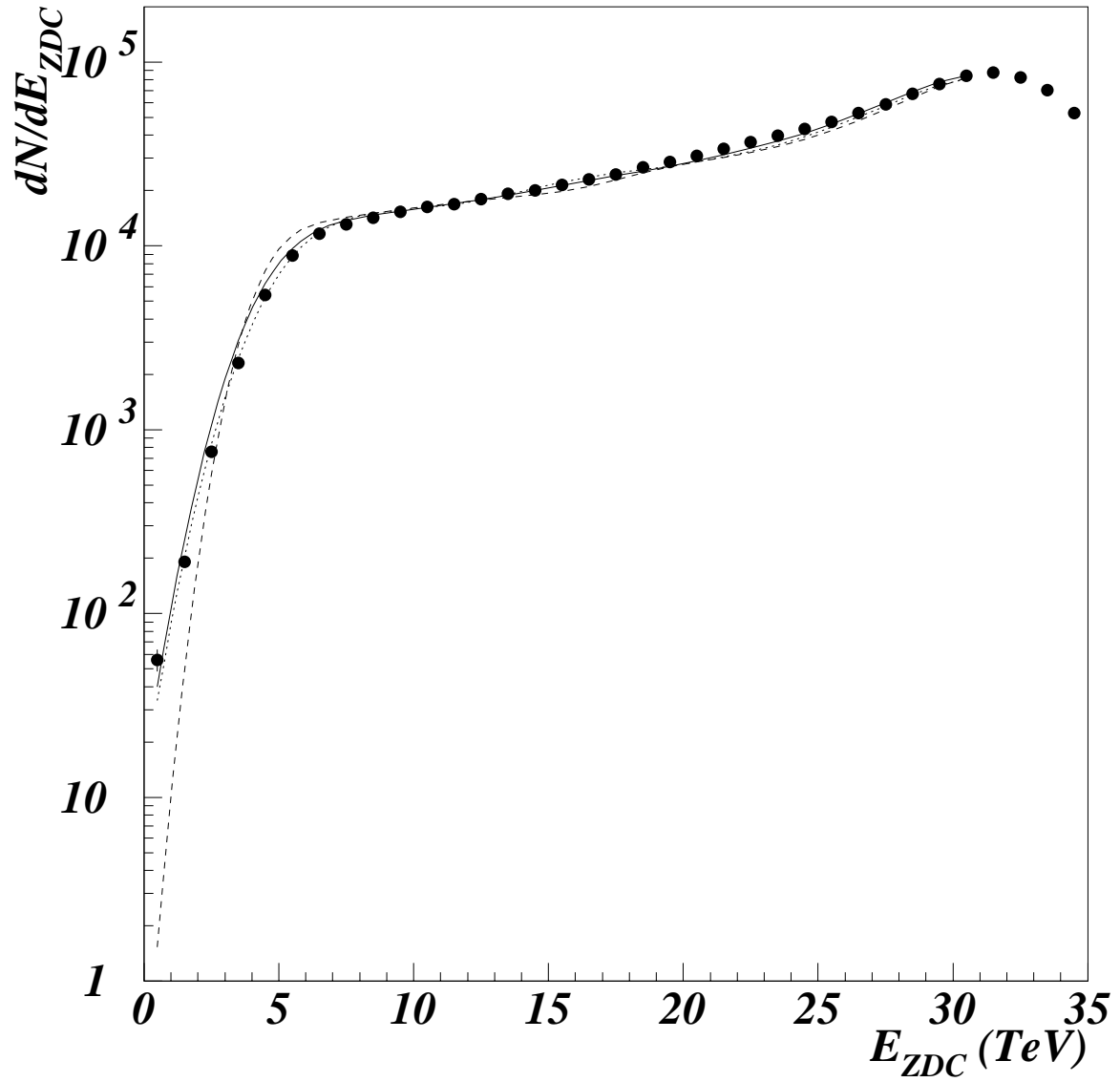
Figure 1: Comparison of the minimum bias E_{ZDC} spectrum with the result of the Glauber calculation (full line), and of the Monte-Carlo simulations based on VENUS (dashed line) and on RQMD (dotted line).
