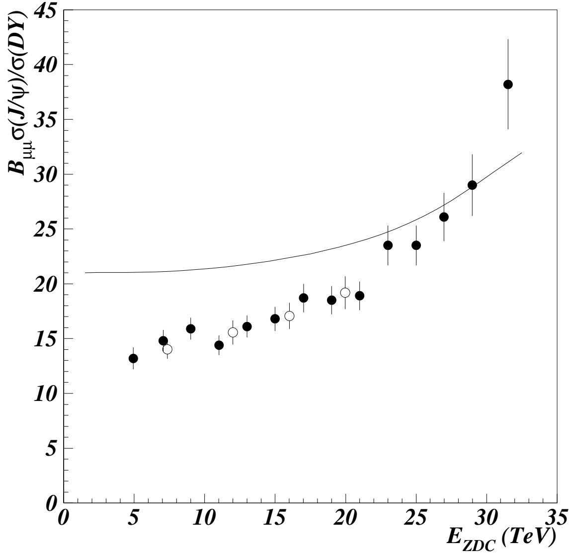
Figure 3: The results of the standard analysis for the 1996 (closed circles) and 1998 (open circles) data samples. The curve represents the results of a Glauber calculation which takes into account the J/\psi suppression due to ordinary nuclear absorption, with \sigma_{J/\psi}^{abs} = 6.4 mb.
