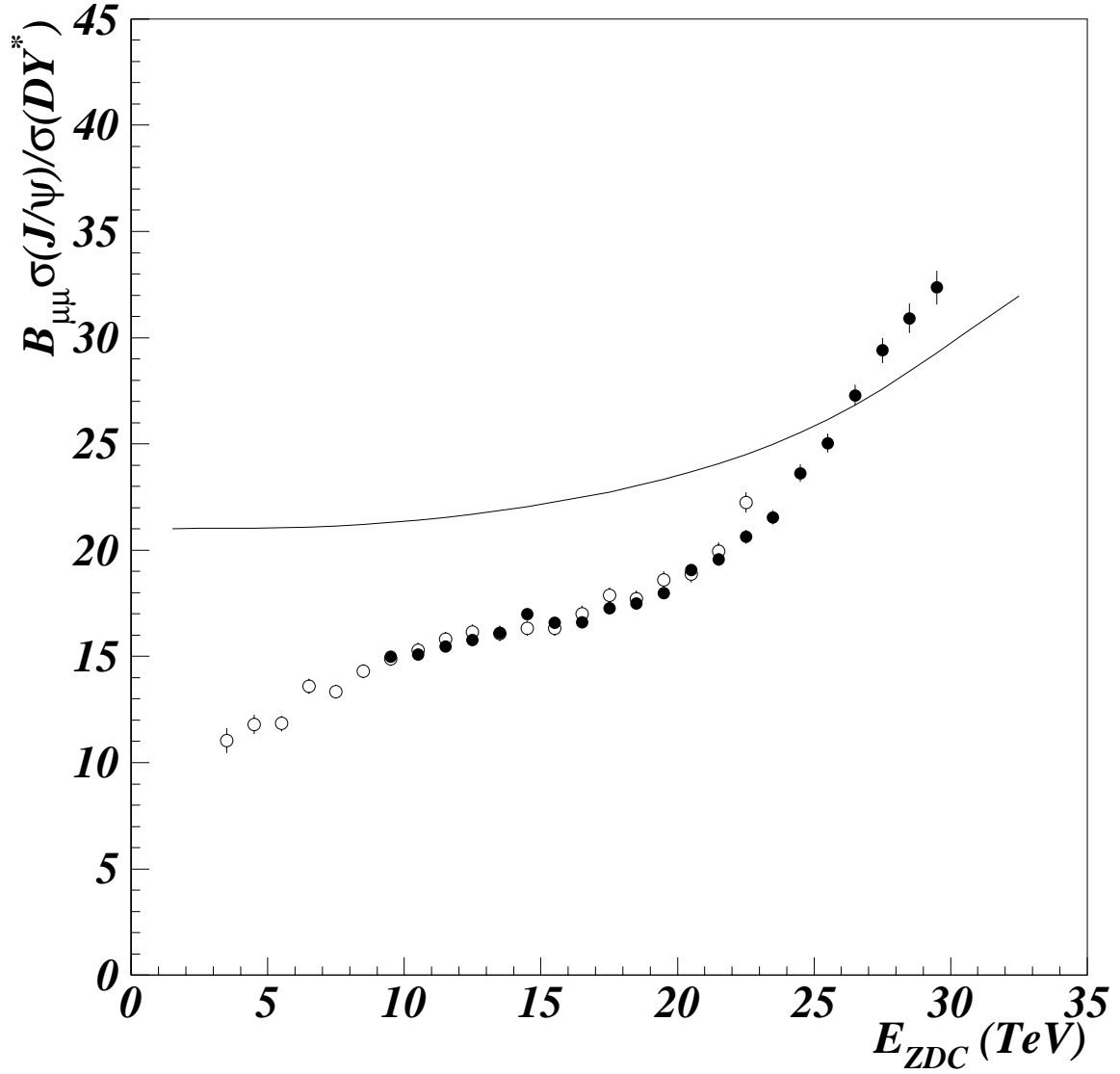
Figure 5: The results of the minimum bias analysis. The full symbols refer to 1996 data and the open symbols to 1998 data. The curve represents the results of a Glauber calculation which takes into account the J/\psi suppression due to ordinary nuclear absorption, with \sigma_{J/\psi}^{\text{abs}} = 6.4 mb.
