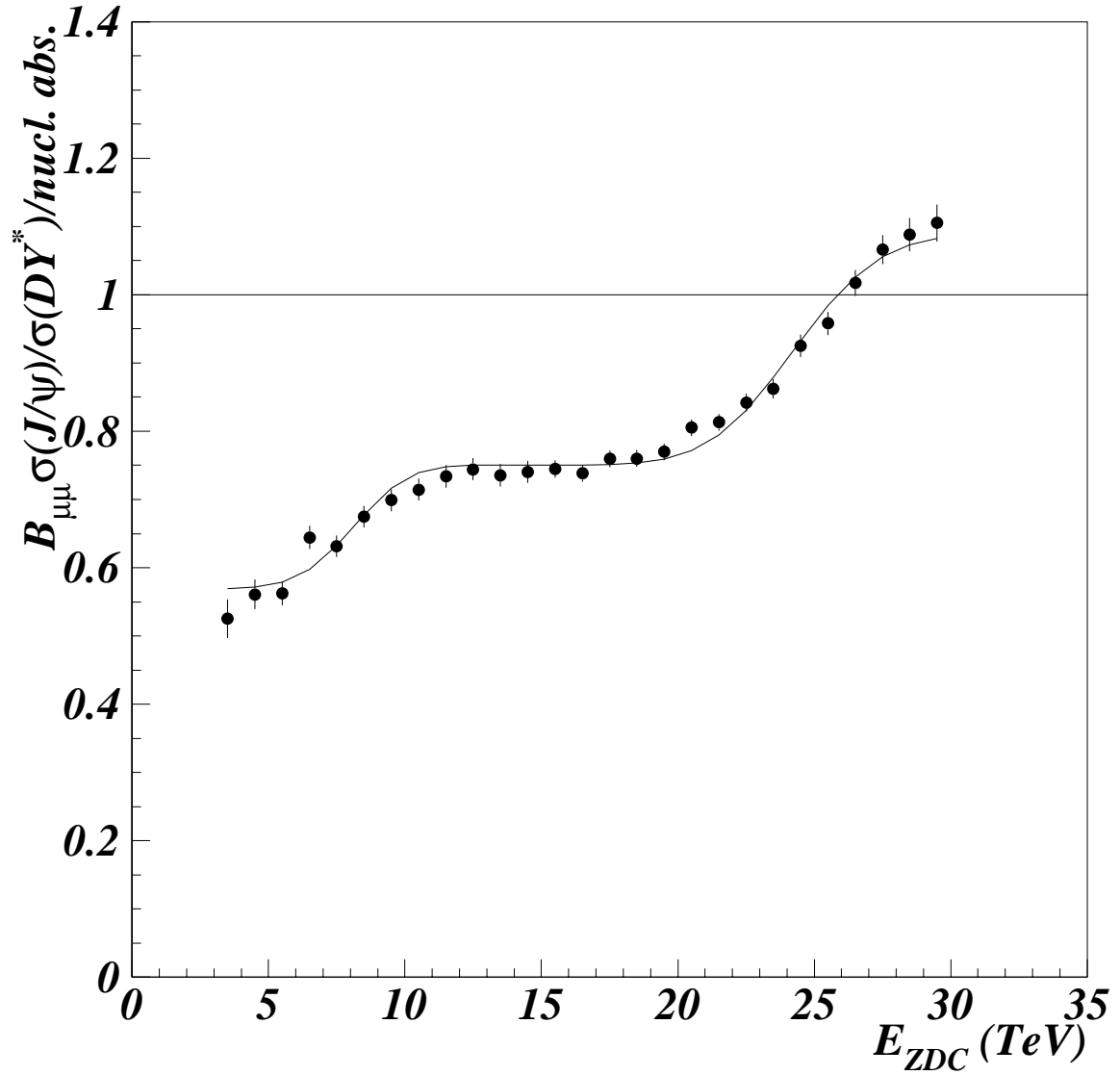
Figure 9: The fit of \sigma_{J/\psi}/\sigma_{DY^*} versus E_{ZDC} , assuming two sharp absorption mechanisms of free amplitude occurring at N_{\text{part}} = 122 and N_{\text{part}} = 334 .
