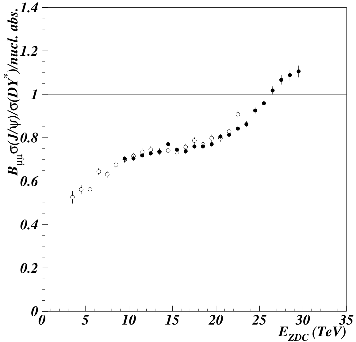
Figure 6: The \sigma_{J/\psi}/\sigma_{DY^*} ratio divided by the absorption curve, as a function of E_{ZDC} . The full symbols refer to the 1996 data and the open symbols to the 1998 data.
