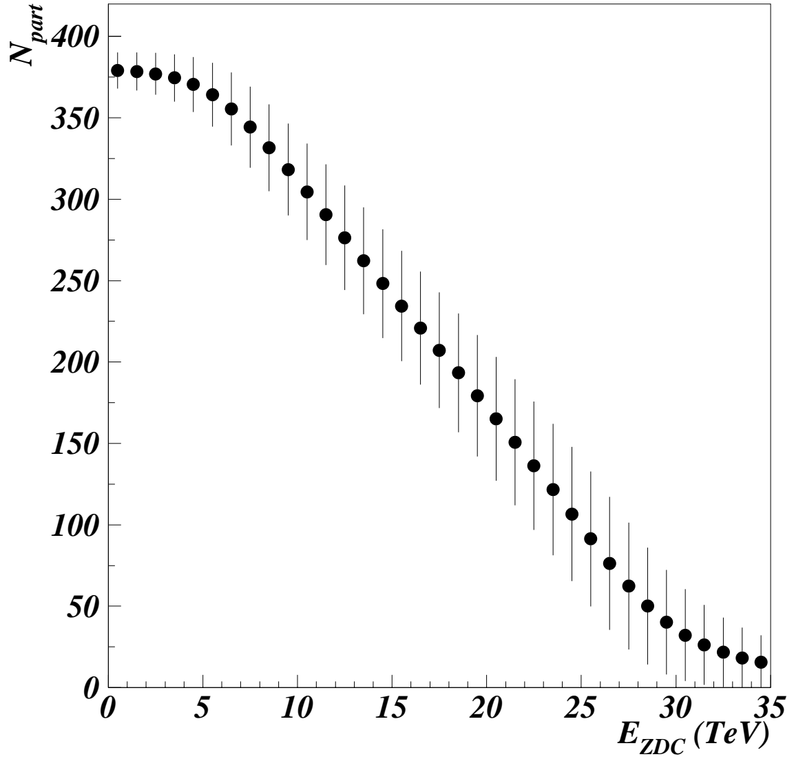
Figure 2: The number of participants N_{part} as a function of E_{ZDC} , calculated in our Glauber approach. The error bars represent the r.m.s. of the N_{part} distribution at fixed E_{ZDC} .
