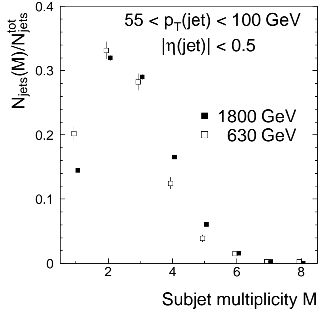
FIG. 18. Uncorrected subject multiplicity in jets from D\bar{D} data at \sqrt{s} = 1800 GeV and 630 GeV.
