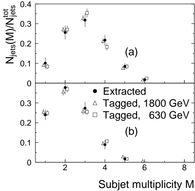
FIG. 17. Uncorrected subject multiplicity in fully-simulated Monte Carlo (a) gluon and (b) quark jets. The number of jets N_{\text{jets}}(M) in each bin of subject multiplicity on the vertical axis is normalized to the total number of jets in each sample N_{\text{jets}}^{\text{tot}} = \sum_M N_{\text{jets}}(M) . The measured distributions (solid) are extracted from the mixed Monte Carlo jet samples at \sqrt{s} = 1800 GeV and 630 GeV. The tagged distributions (open) are for \sqrt{s} = 1800 GeV (triangles) and 630 GeV (squares).
