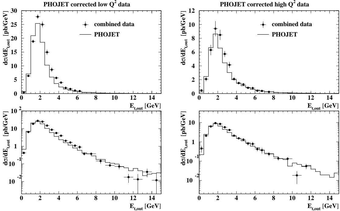
Figure 19: The combined E_{t,out} distribution from ALEPH, L3 and OPAL for the low- Q^2 (left) and high- Q^2 region(right), corrected with and compared to the PHOJET model.
