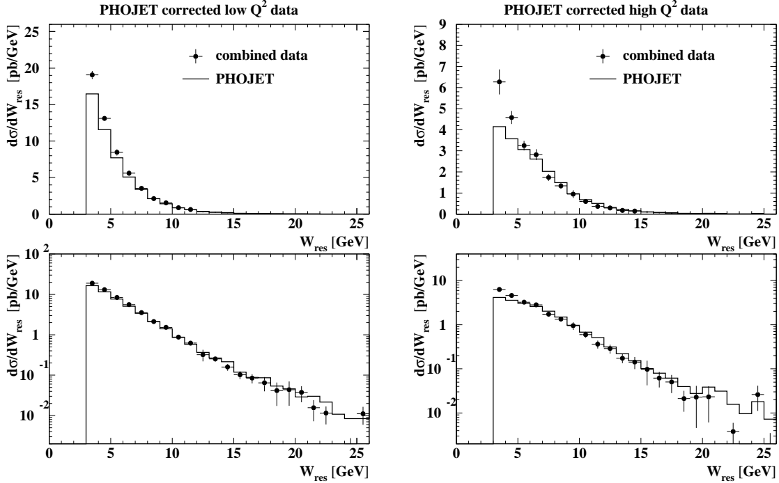
Figure 17: The combined W_{\text{res}} distribution from ALEPH, L3 and OPAL for the low- Q^2 (left) and high- Q^2 region (right), corrected with and compared to the PHOJET model.
