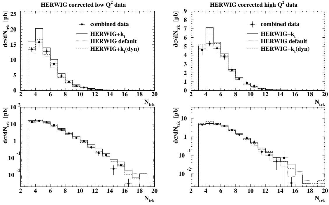
Figure 20: The combined N_{\text{trk}} distribution from ALEPH, L3 and OPAL for the low- Q^2 (left) and high- Q^2 region (right), corrected with the HERWIG+ k_t model on a linear scale (top) and on a log scale (bottom). The data are compared to three different model assumptions of the HERWIG+ k_t model.
