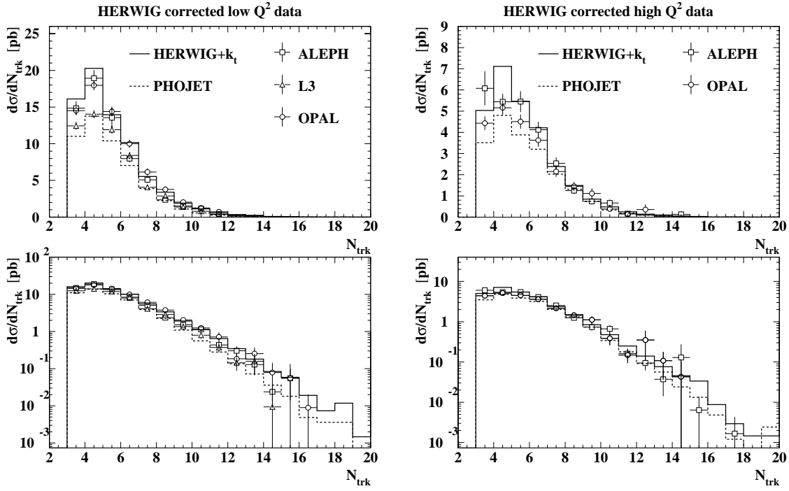
Figure 10: The N_{\text{trk}} distributions from ALEPH, L3 and OPAL for the low- Q^2 (left) and high- Q^2 region (right), corrected with the HERWIG+ k_t model on a linear scale (top) and on a log scale (bottom).
