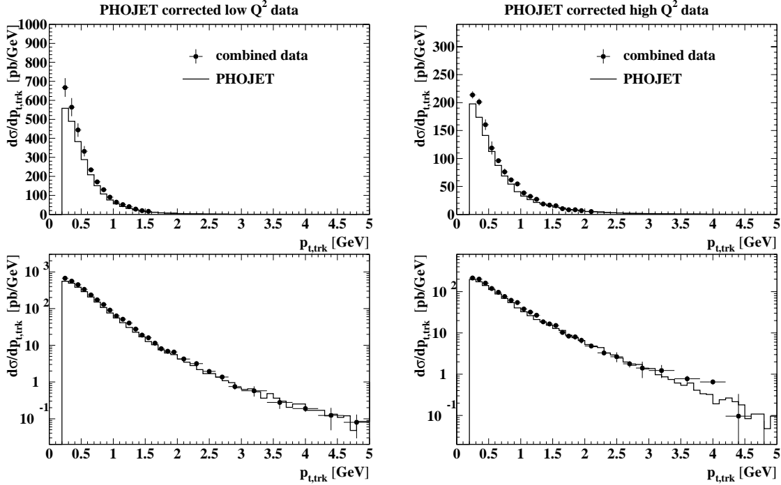
Figure 23: The combined p_{t,\text{trk}} distribution from ALEPH, L3 and OPAL for the low- Q^2 (left) and high- Q^2 region (right), corrected with and compared to the PHOJET model.
