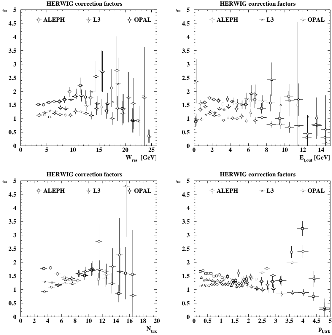
Figure 4: The HERWIG+ k_t correction factors, f , for the ALEPH, L3 and OPAL W_{\text{res}} , E_{t,\text{out}} , N_{\text{trk}} and p_{t,\text{trk}} distributions for the low- Q^2 region. The symbols are slightly displaced for better visibility.
