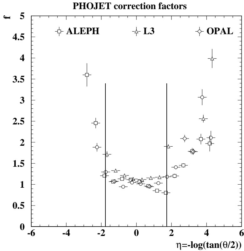
Figure 3: The HERWIG+ k_t and PHOJET correction factors, f , for the ALEPH, L3 and OPAL energy flow for the low- Q^2 region. The symbols are slightly displaced for better visibility. The vertical lines indicate the central rapidity region, |\eta| < 1.735 .
