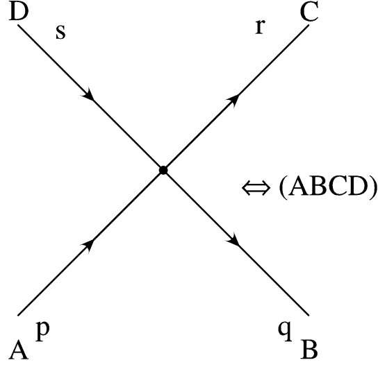
Figure 18: Four-particle vertex.
