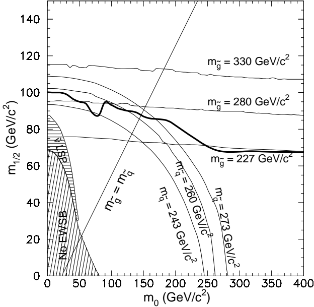
FIG. 2. Exclusion contour in the (m_0, m_{1/2}) plane for \tan\beta = 2 , \mu < 0 , A_0 = 0 , and finite \lambda'_{2jk} ( j = 1, 2 ; k = 1, 2, 3 ) coupling. The region below the bold line is excluded at the 95% C.L. The cross hatched region is excluded for theoretical reasons (see text). m_{\tilde{q}} and m_{\tilde{g}} denote the squark and gluino masses, respectively.
