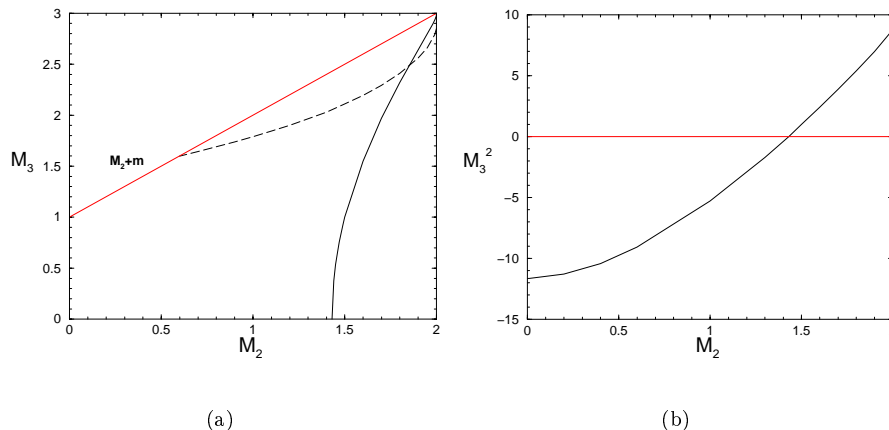
Figure 1. (a) Three-body bound state mass M_3 v.s. the two-body one M_2 . Solid line corresponds to present work, dash line and dots – to calculations using the integration limits of [3]. (b) Three-body bound state mass squared M_3^2 v.s. M_2 .
