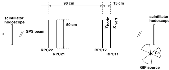
Fig. 3. Sketch of the experimental setup of the mini-trigger experiment.
