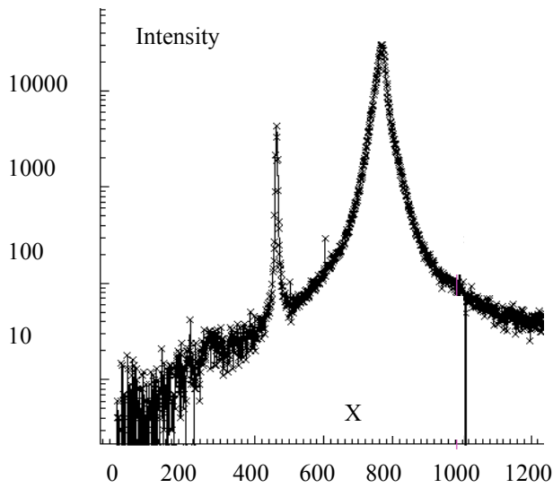
Fig. 1. CCD Bragg diffraction image.
