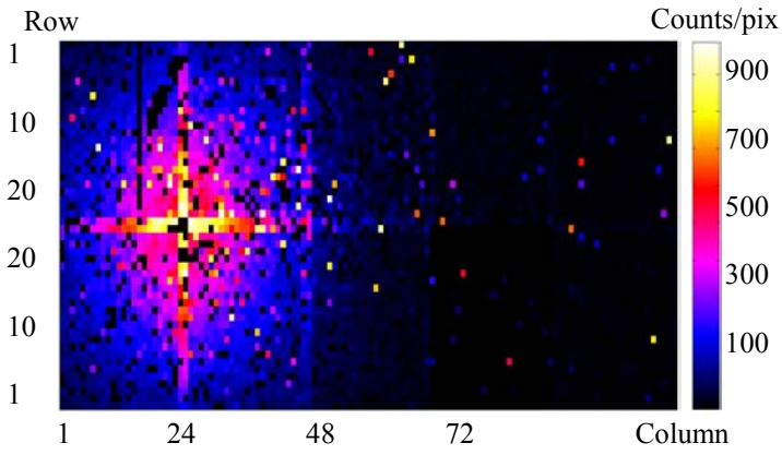
Fig. 6. Beam profile of a Sr^{90} source placed on a module prototype, in the middle of 4 chips (the cross is due to the larger pixels in this area)
