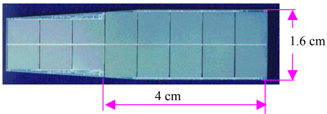
Fig. 2. DELPHI pixel detector
