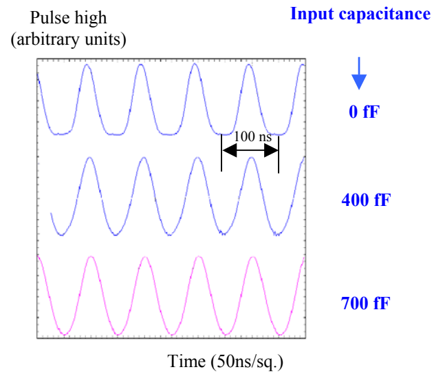
Fig. 5. Amplifier output with 10^7 pulse/sec, for three input capacitance's.
