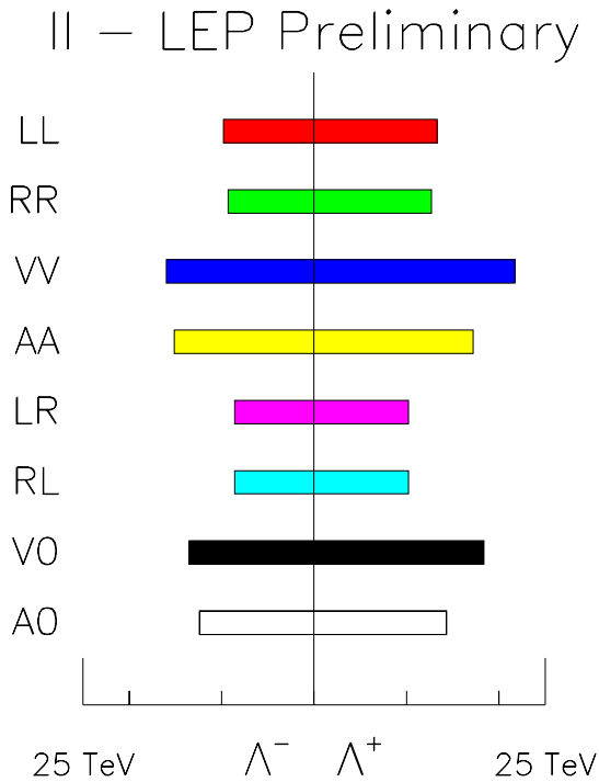
Fig. 2. Limits on the scale of CI in e^+e^- \rightarrow \mu^+\mu^- + \tau^+\tau^- using LEP combined measurements from 130 to 209 GeV
