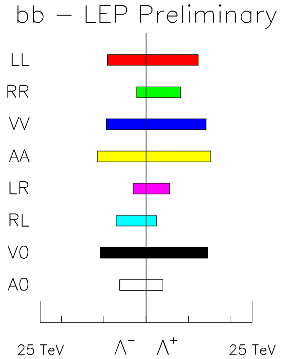
Fig. 3. Limits on the scale of CI in e^+e^- \rightarrow b\bar{b} using LEP combined measurements from 130 to 209 GeV
