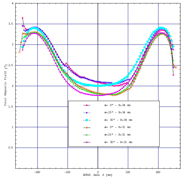
Figure 5 : Total magnetic field along the ECRIS axis for several radius and azimuthal angles.
