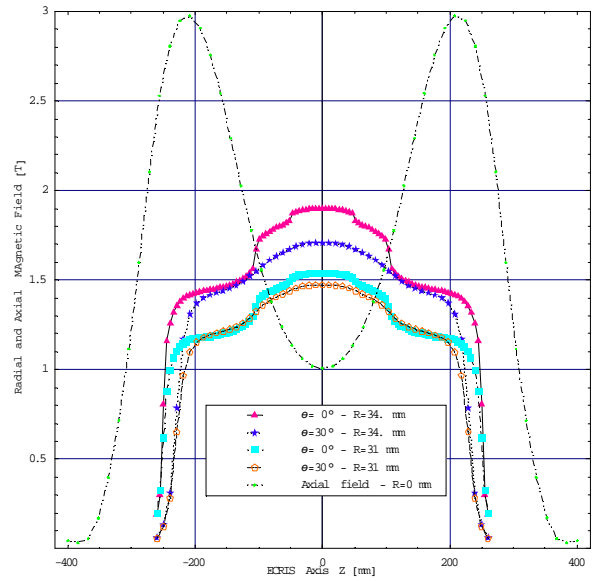
Figure 3 : Radial Magnetic confinement along the axis of ECRIS axis in front of the magnets (R=34 mm) and at the inner edge of the plasma chamber (R=31 mm). Last plot is the Axial magnetic profile at R=0 with a current density of 80 A/mm 2 in each coil.
