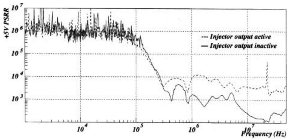
Figure 7: Power supply rejection ratios (PSRR) on the -5 V (top) and +5 V (bottom) lines of a DMILL BiCMOS injector
