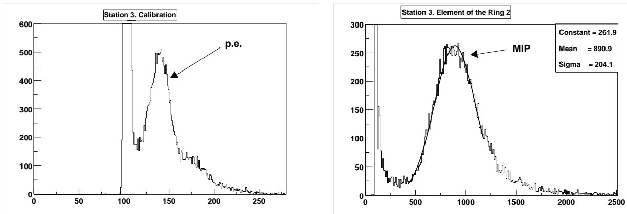
Figure 7: Charge distributions provided by a XP2020 photo-multiplier from the one photo-electron (left) and from the one MIP (right) through a counter of the ring 2.
