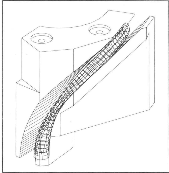
Figure 2 : Beam envelope through the Müller inflector, using the CHA3D solver and the PELLCE dynamic code.
