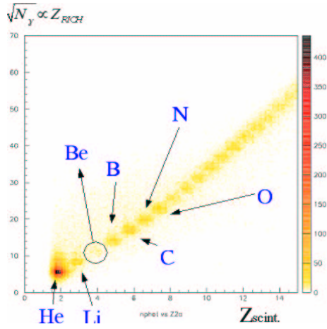
Fig. 5. Correlation between a dE/dX scintillator and the square root of the number of Cherenkov photons
