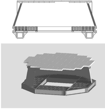
Fig. 1. Structure of the final imager
