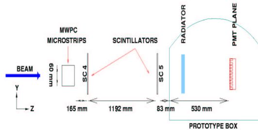
Fig. 4. Experimental setup on the beam line
