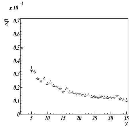
Fig. 7. Velocity resolution vs charge
