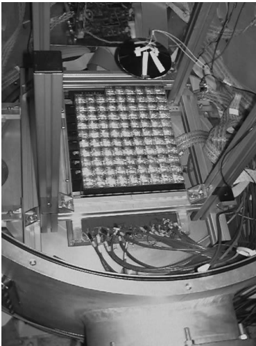
Fig. 2. Prototype matrix in its light tight box
