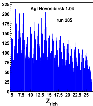
Fig. 8. Charge reconstruction for n=1.04 CIN Aerogel
