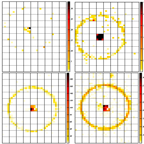
Fig. 6. Ring patterns for Z = 2 (top left), 6 (top right), 10 (bottom left) and around 26 (bottom right)
