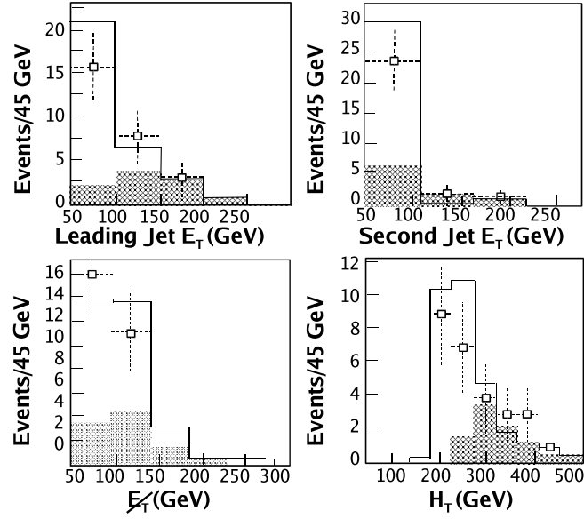
FIG. 1: Data (points) and predicted background (histograms) after final selections. The additional contributions expected from a M_{\tilde{t}}=130 \text{ GeV}/c^2 , M_{\tilde{\chi}_1^0}=30 \text{ GeV}/c^2 scalar top quark are shown by shaded histograms. The plots correspond to the E_T of the leading jet, second jet, \cancel{E}_T (the three parameters optimized using the RGS) and H_T , where H_T = \cancel{E}_T + \sum_i E_T(\text{jet}_i) , to demonstrate agreement with variables not directly optimized via RGS.
