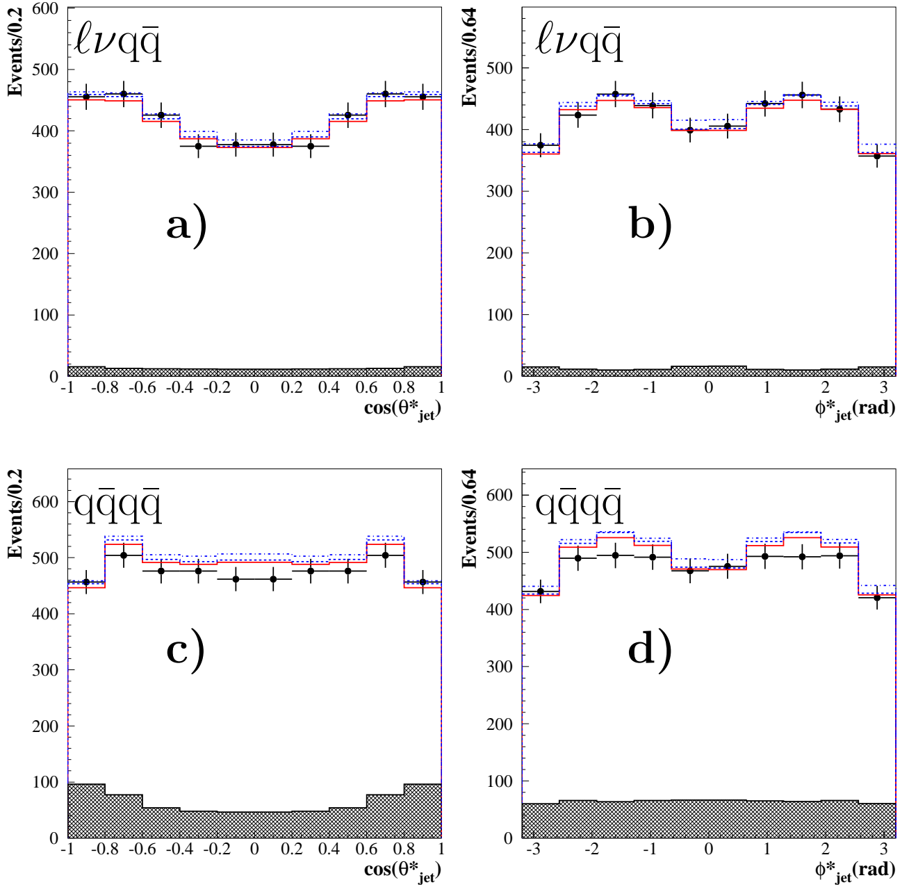
Figure 3: Distributions of the polar and azimuthal angles, \cos\theta_{jet}^* and \phi_{jet}^* , of the jets in the rest frame of its parent W for l\nu q\bar{q} a) and b) and for q\bar{q}q\bar{q} c) and d). Within a W boson, the choice between quark and anti-quark jets is ambiguous. The two (four) possible choices are filled in the histogram with a weight of 0.5 for the l\nu q\bar{q} channel (0.25 for the q\bar{q}q\bar{q} channel). Data are represented by solid dots. The solid line shows the Standard Model prediction while dashed and dashed-dotted histograms display the effect of \lambda_\gamma = +0.2 and \lambda_\gamma = -0.2 . The background contribution is represented by the hatched area.
