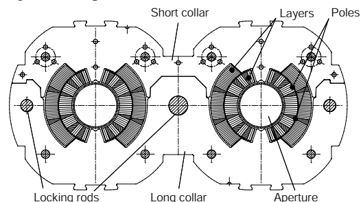
Fig. 1: Collared coil cross section
