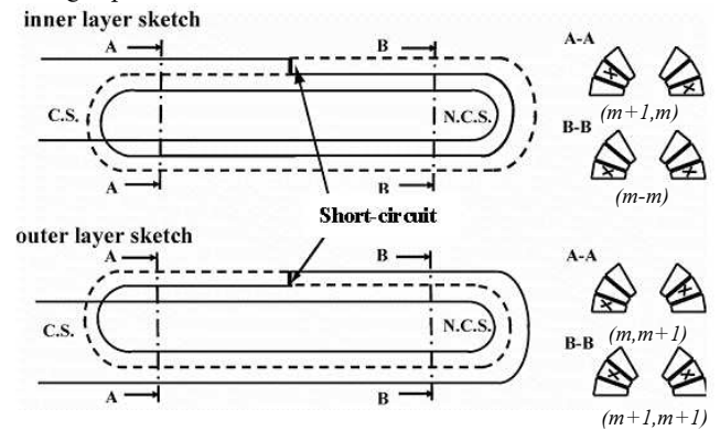
Fig. 2: Simplified model of a coil with two layers of three cable turns; dashed line is the turn bypassed by the current (left). Cross sections of the coils with respect to the short: the crosses indicate that no current is flowing inside the cable (right).
