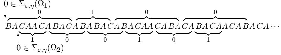
Figure 3: Block structure of quasisturmian words.
