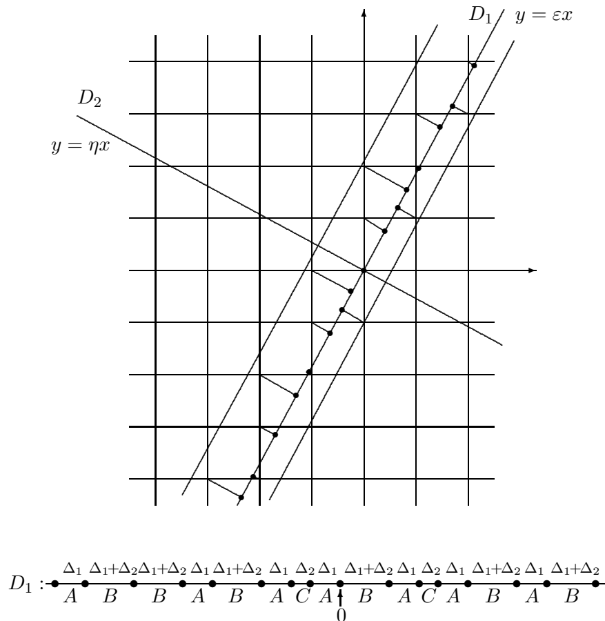
Figure 1: Construction of a cut-and-project sequence and assignment of the infinite word which codes the order of distances in the cut-and-project sequence.
