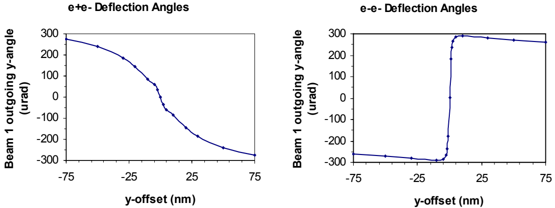
Figure 2: Vertical deflection angle (beam 1) versus vertical offset for e^+e^- and e^-e^- collisions at the ILC with nominal parameters at 500 GeV in the centre-of-mass.
