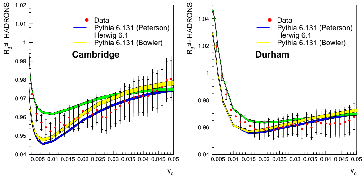
Figure 7: R_3^{b\ell} at hadron level as a function of y_c compared with PYTHIA 6.131 (with Peterson and Bowler fragmentation b functions) and HERWIG 6.1 predictions, using the CAMBRIDGE (left) and DURHAM (right) jet-clustering algorithms.
