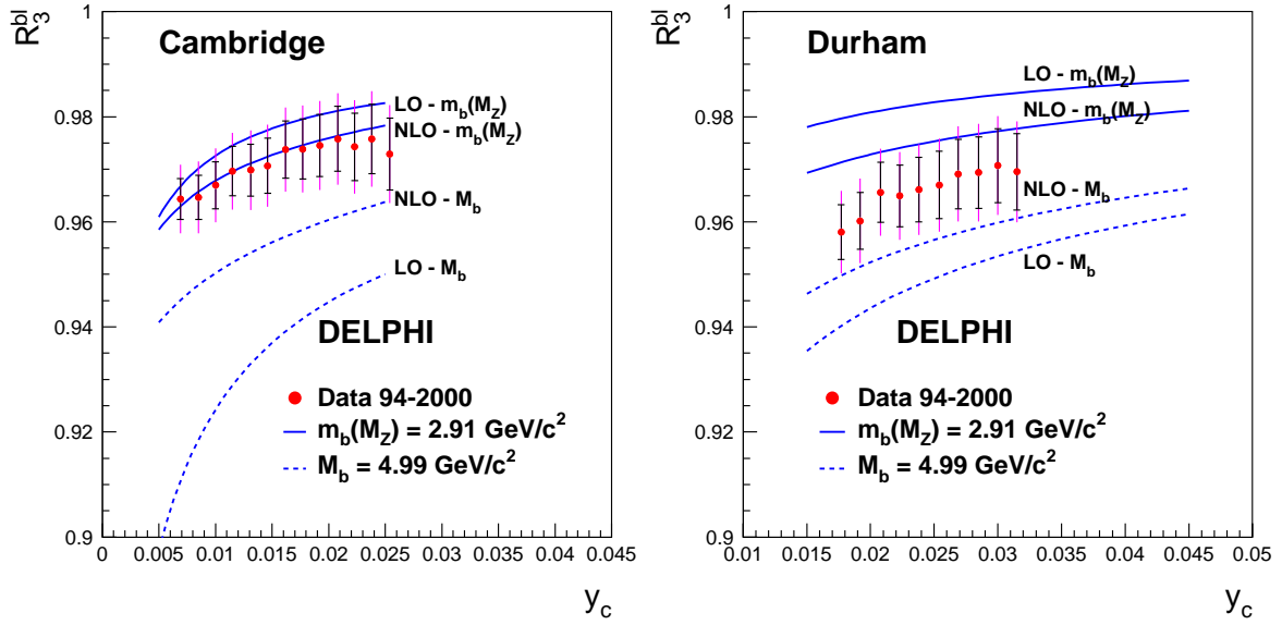
Figure 8: R_3^{bl} as a function of y_c obtained at parton level compared with the LO and NLO theoretical predictions calculated in terms of a pole mass of M_b = 4.99 \text{ GeV}/c^2 and in terms of a running mass of m_b(M_Z) = 2.91 \text{ GeV}/c^2 .
