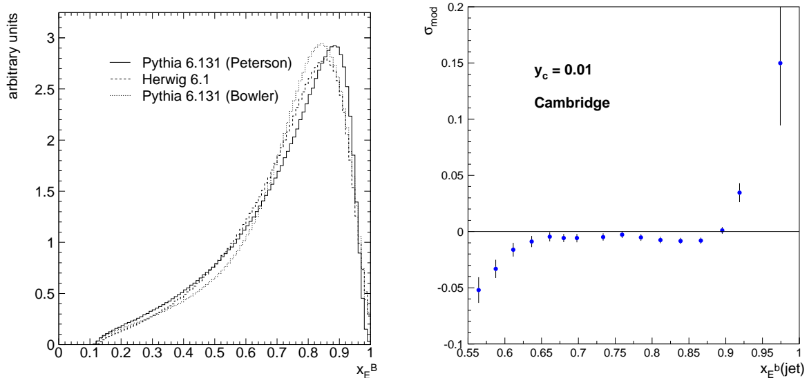
Figure 1: x_E^B distribution for the different Monte Carlo generators (left). Hadronization model uncertainty (i.e. standard deviation of the hadronization corrections predicted by HERWIG and PYTHIA with Peterson and Bowler heavy fragmentation functions) as a function of the mean of the x_E^b(\text{jet}) that is defined in the text and for y_c = 0.01 for CAMBRIDGE (right).
