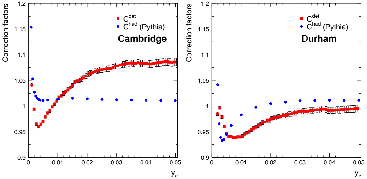
Figure 6: Detector and hadronization corrections applied to the measured R_3^{b\ell} for CAMBRIDGE and DURHAM. The detector correction, C^{det} , brings the observable to hadron level, and the hadronization correction, C^{had} , brings it from this stage to parton level.
