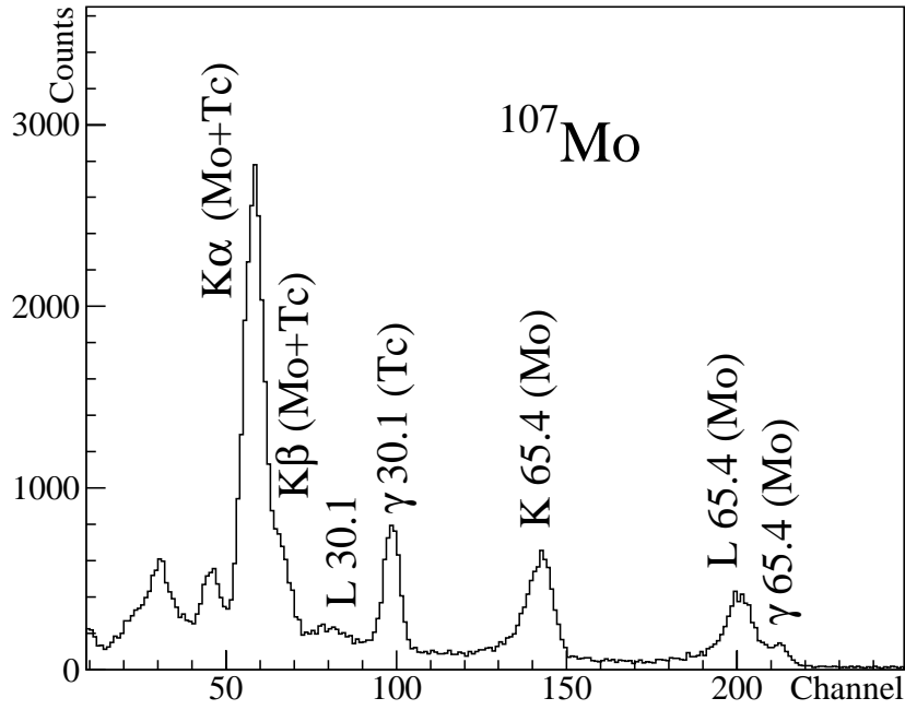
FIG. 6: Si(Li) spectrum of the A=107 isomers observed in the present experiment. Narrow peaks correspond to X- and \gamma -rays, while the broader peaks are due to conversion electrons.
