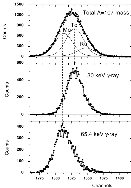
FIG. 5: Comparison of the energy lost by the FFs of mass A=107 in the first region of gas of the ionization chamber, in three different cases: a) without any conditions, b) in coincidence with the 30 keV transition and c) in coincidence with the 65.4 keV transition. In a) the spectra of the three main isotopes contributing to the A=107 mass are also reported. It is clearly evidenced in this figure that the 30 keV and 65.4 keV transitions belong to Tc and Mo, respectively.
