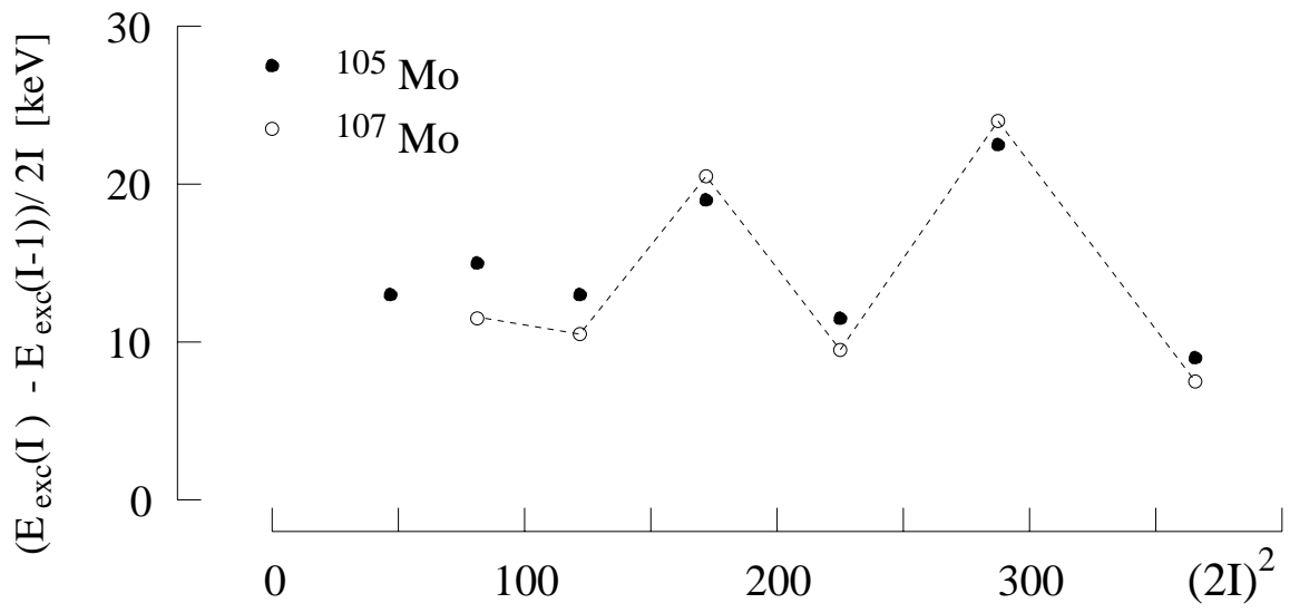
FIG. 3: Staggering in the negative-parity bands of ^{105}\text{Mo} and ^{107}\text{Mo} [5]. The dashed line is drawn to guide the eye.
