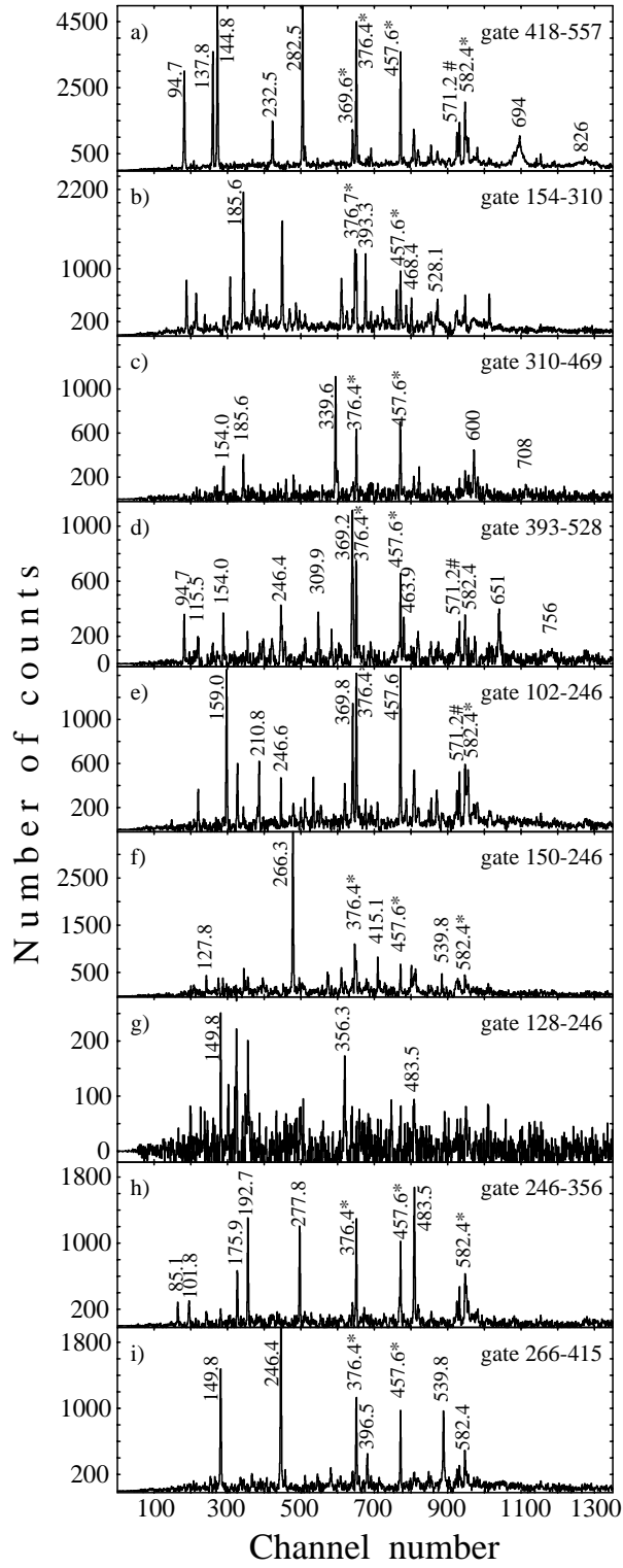
FIG. 2: Coincidence spectra gated on \gamma -lines in ^{105}\text{Mo} . Energies of lines are given in keV. Symbol “*” denotes lines in ^{140}\text{Xe} . Unlabelled lines are from contaminating nuclei.
