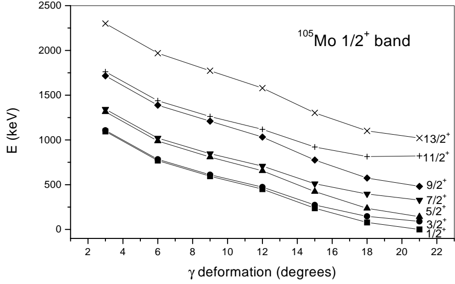
FIG. 8: Variation of the theoretical energy levels of the 1/2^+ band in ^{105}\text{Mo} as function of \gamma deformation.
