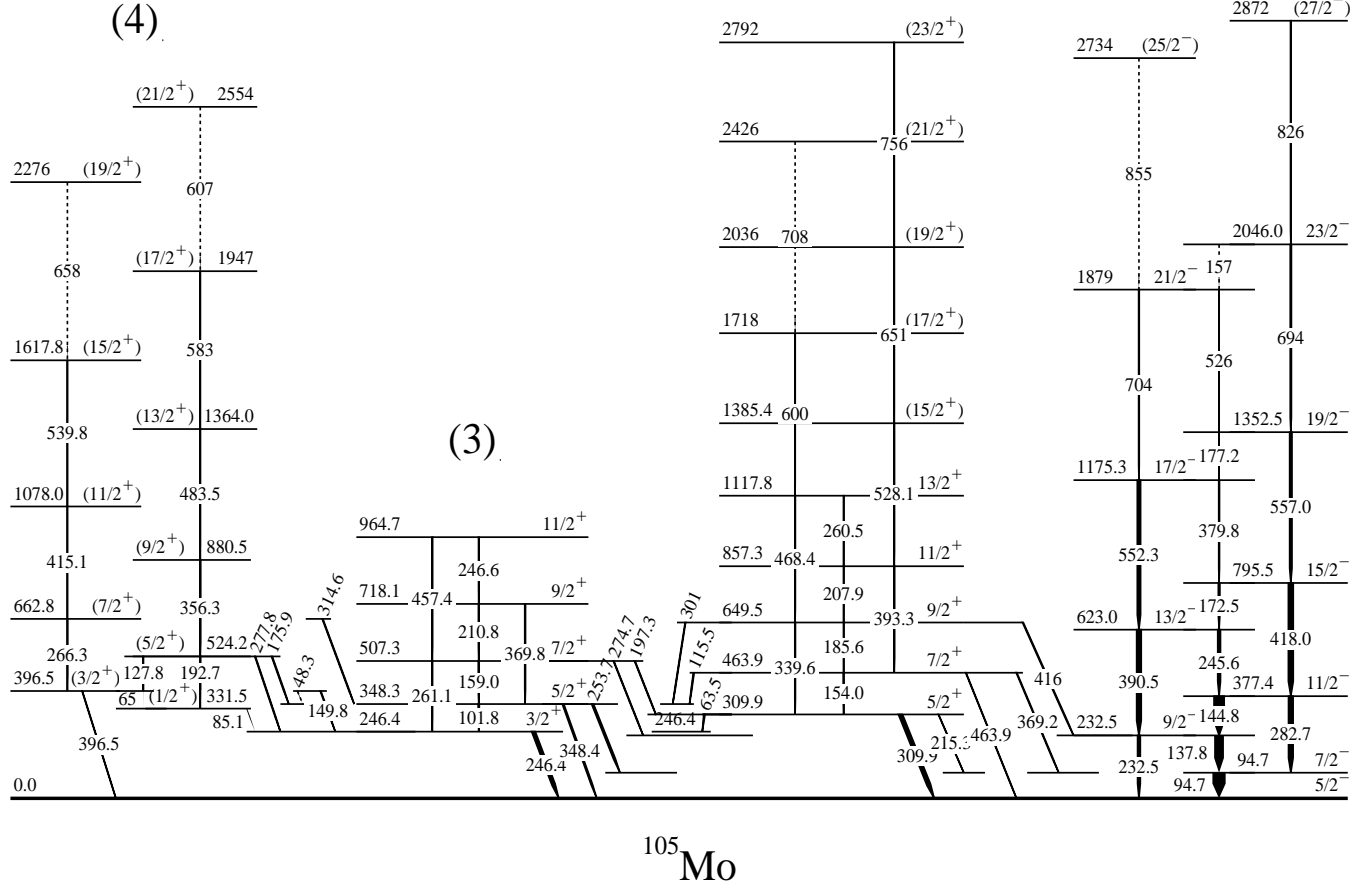
FIG. 1: Partial level scheme of ^{105}\text{Mo} as obtained in this work. Arrow thickness is proportional to the relative \gamma intensities of transition. Uncertainties on \gamma energies are from 0.1 keV for strong lines and up to 0.5 keV for weak lines.
