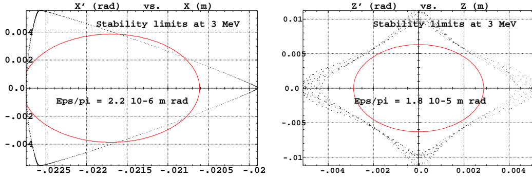
FIG. 14 – Stability limits at 3 MeV and their corresponding acceptances left for horizontal motion and right for vertical motion.
