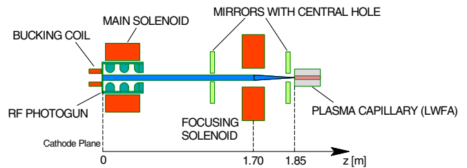
FIG. 1. (Color) Schematic of the Alpha-X setup.
