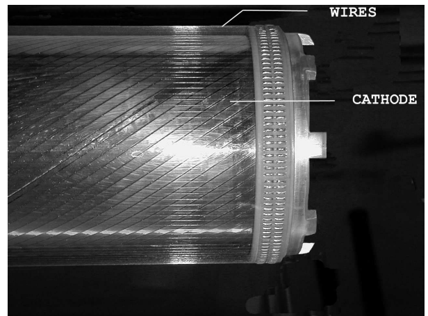
Fig. 3. Detailed view of the tip of the internal cylindrical chamber showing the helicoidal strips and the wires. The pitch angle of the strips is 34^\circ .
