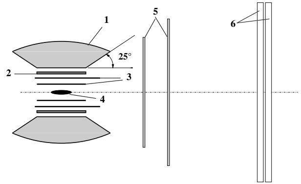
Fig. 1. Schematic view of the LA \gamma RANGE detector: BGO calorimeter (1), Plastic scintillator (2), Cylindrical MWPC's (3), Target (4), Plane MWPC's (5), Double plastic scintillator hodoscope (6) (the drawing is not to scale).
