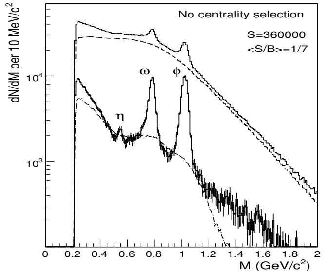
Figure 2. Raw mass distribution (continuous line), fake tracks (dot-dashed line), combinatorial background (dashed line) and mass distribution after fake tracks and combinatorial background subtraction (continuous curve with error bars).
