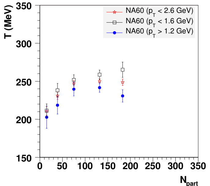
Figure 6. T slope parameter as a function of the number of participants, estimated in three different p_T windows. Statistical errors only.
