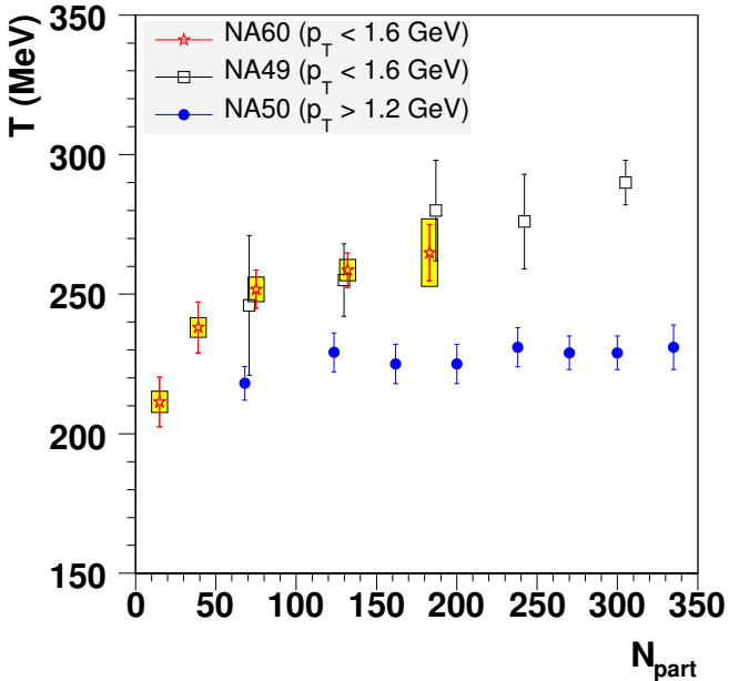
Figure 7. T slope parameter as a function of the number of participants (open red stars). Fit performed in the range 0.0 \text{ GeV} < p_T < 1.6 \text{ GeV} . Compared to the T slope measured in Pb-Pb collisions by the NA49 experiment (open black squares) and NA50 experiment (full blue circles). The boxes show the systematic error.
