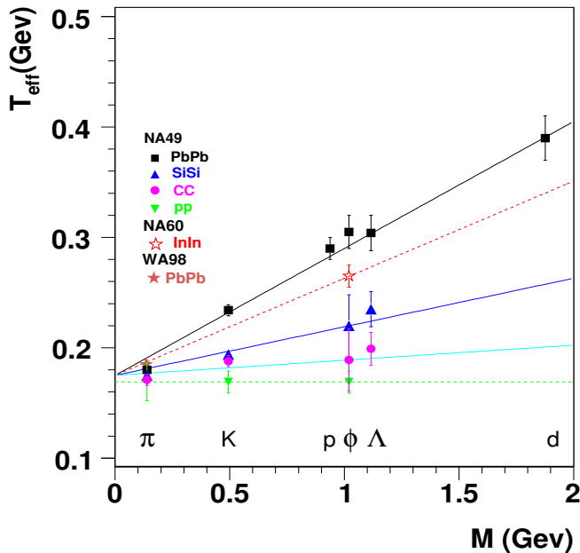
Figure 9. T slope parameter as a function of particle mass for central events in several collision systems. The NA60 data point was obtained from a fit in the range 0.0 \text{ GeV} < p_T < 1.6 \text{ GeV} .
