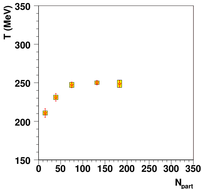
Figure 5. T slope parameter as a function of the number of participants. Fit performed in the range 0.0 \text{ GeV} < p_T < 2.6 \text{ GeV} . The boxes show the systematic error.
