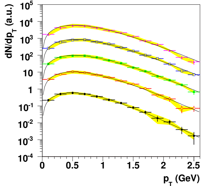
Figure 4. \phi transverse momentum distributions in indium-indium collisions as a function of centrality. From top to bottom: central to peripheral spectra. The band shows the systematic error.
