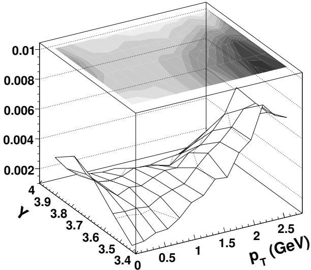
Figure 3. Acceptance times reconstruction efficiency in central In-In collisions for the \phi meson mass.
