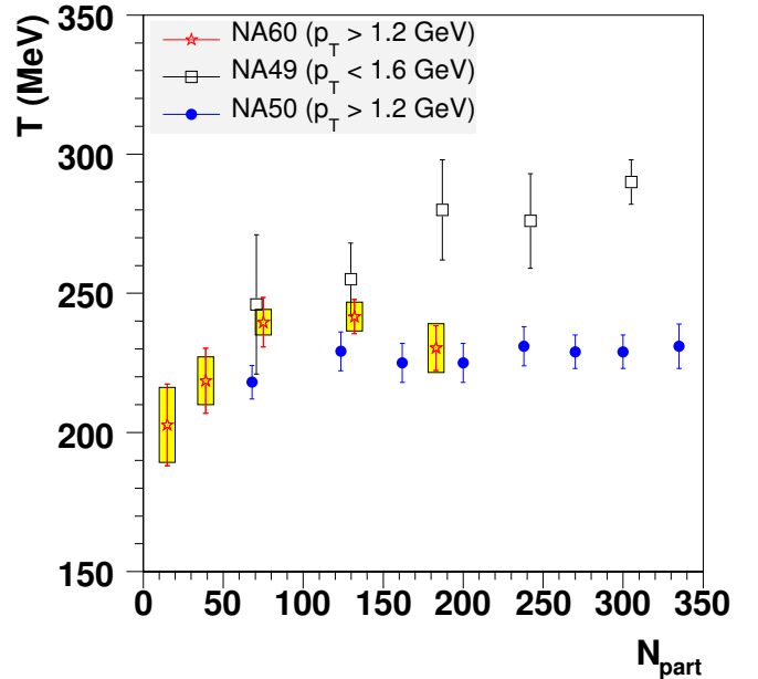
Figure 8. T slope parameter as a function of the number of participants (open red stars). Fit performed in the range 1.2 \text{ GeV} < p_T < 2.6 \text{ GeV} . Compared to the T slope measured in Pb-Pb collisions by the NA49 experiment (open black squares) and NA50 experiment (full blue circles). The boxes show the systematic error.
