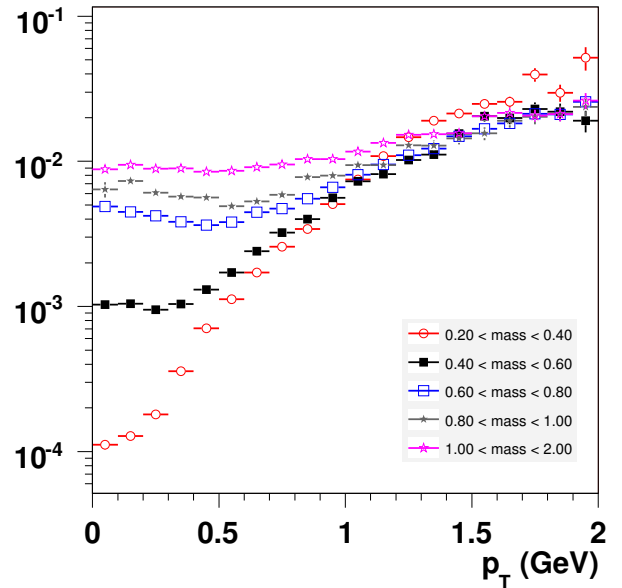
Figure 1. Dimuon geometrical acceptance as a function of p_T in several mass windows.
