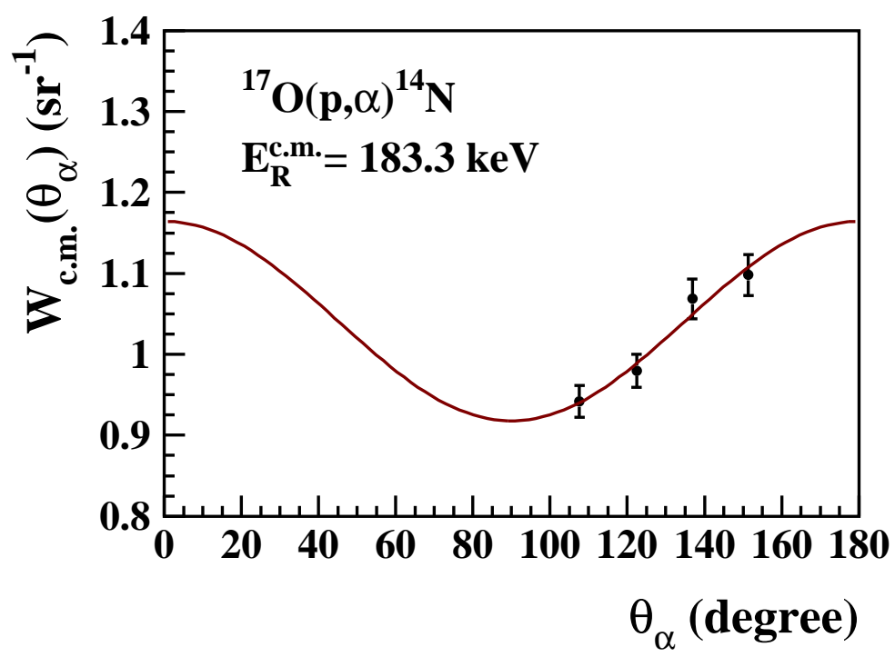
FIG. 5: (Color online) Angular distribution (center of mass) for the ^{17}\text{O}(p,\alpha)^{14}\text{N} resonance at E_{\text{c.m.}}=183.3 \text{ keV} . The solid line shows a Legendre-polynomial fit to the data points, W_{\text{c.m.}}(\theta_{\alpha}) = 1 + a_2 P_2(\cos\theta_{\alpha}) , which yields a_2=0.16\pm 0.03 .
