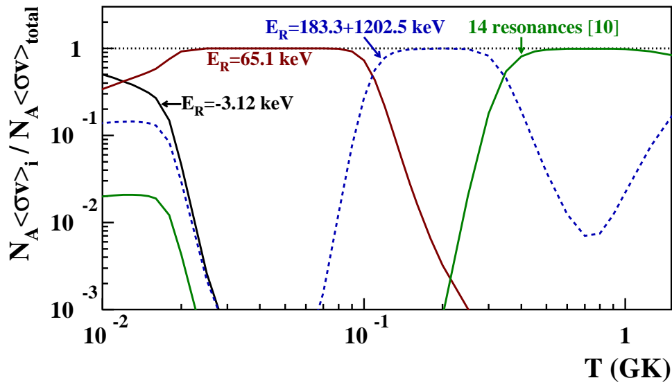
FIG. 8: (Color online) Ratios of individual reaction rate contributions to the total modal rate for the ^{17}\text{O}(p,\alpha)^{14}\text{N} reaction. The unlabelled solid and dashed lines below 0.02 GK correspond to tail contributions of the resonances at 0.557+0.677 MeV and 1.202 MeV, respectively (see text).
