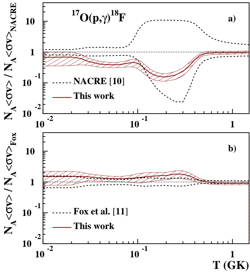
FIG. 12: (Color online) Comparison of present and previous reaction rates for the ^{17}\text{O}(p,\gamma)^{18}\text{F} reaction. In part a (b) is given the ratio of the present rates to the rates evaluated in Ref. [10] (Ref. [11]). The hatched area gives the present uncertainties in the reaction rates. Upper and lower limits for the rates of Refs. [10, 11] are given as dashed lines.
