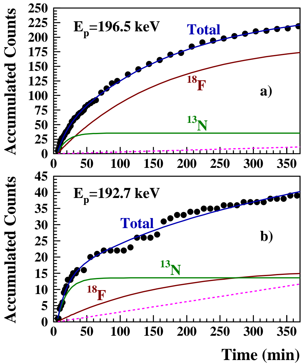
FIG. 7: (Color online) Measured \beta^+ activities of two ^{17}\text{O} -implanted targets irradiated at (a) E_p^{\text{lab}}=196.5 keV (on-resonance) and (b) E_p^{\text{lab}}=192.7 keV (off-resonance). The time origin corresponds to the stopping of the proton irradiation. Also shown are the fitted ^{18}\text{F} and ^{13}\text{N} decay curves (solid lines) and the measured background radiation (dashed lines).
