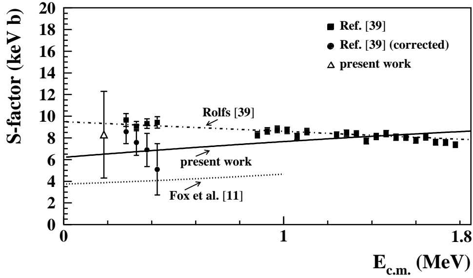
FIG. 10: Previous [11, 39] and present estimates of the direct capture S-factor in the ^{17}\text{O}(p,\gamma)^{18}\text{F} reaction for E_{c.m.}=0 –1.8 MeV. The data points are from Ref. [39] and the present work (triangle at E_{c.m.}=180.2 keV). The four squares at low energy ( <0.45 MeV) are original data from Ref. [39] and circles are corrected low-energy values (see text). The 19 data points above E_{c.m.}=0.88 MeV are representative of the larger number of measured values, which cannot be accurately extracted from Fig. 17 of Ref. [39]. They were generated from a draw in a band around the best estimated value [39] of the DC S-factor (dot-dashed line) with a distribution (and error bars) in accordance with the data spread appreciated from Fig. 17 of Ref. [39]. The solid line shows the present calculations of the DC S-factor, whereas dot-dashed and dotted lines are the previous calculations from Refs. [39] and [11], respectively (see text). Note that the upturn of the S-factor at energies below 0.1 MeV visible in Fig. 17 of Ref. [39] has no influence on the fit and was not considered.
