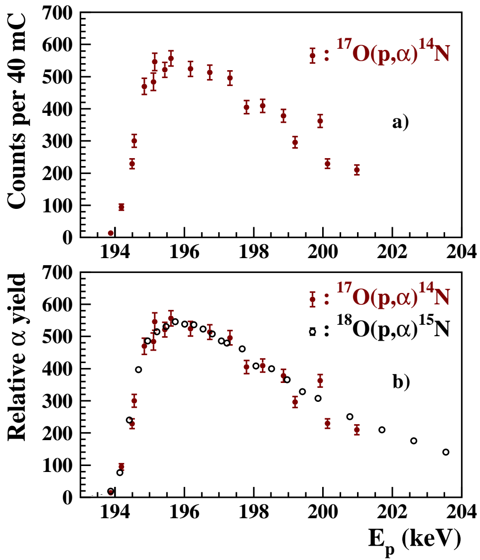
FIG. 6: (Color online) (a) Excitation function for the newly observed resonance at E_R^{\text{lab}}=194.1 keV in the ^{17}\text{O}(p,\alpha)^{14}\text{N} reaction. Yields are given by the sum of the number of counts observed in each of the four detectors normalized according to the measured angular distribution. (b) Comparison of excitation functions for the new resonance at E_R^{\text{lab}}=194.1 keV in the ^{17}\text{O}(p,\alpha)^{14}\text{N} reaction (filled symbols) and the well-known ^{18}\text{O}(p,\alpha)^{15}\text{N} resonance at E_R^{\text{lab}}=150.9 keV (empty symbols). The data for the latter resonance were appropriately normalized and shifted in energy to be compared with those obtained with the ^{17}\text{O} target.
