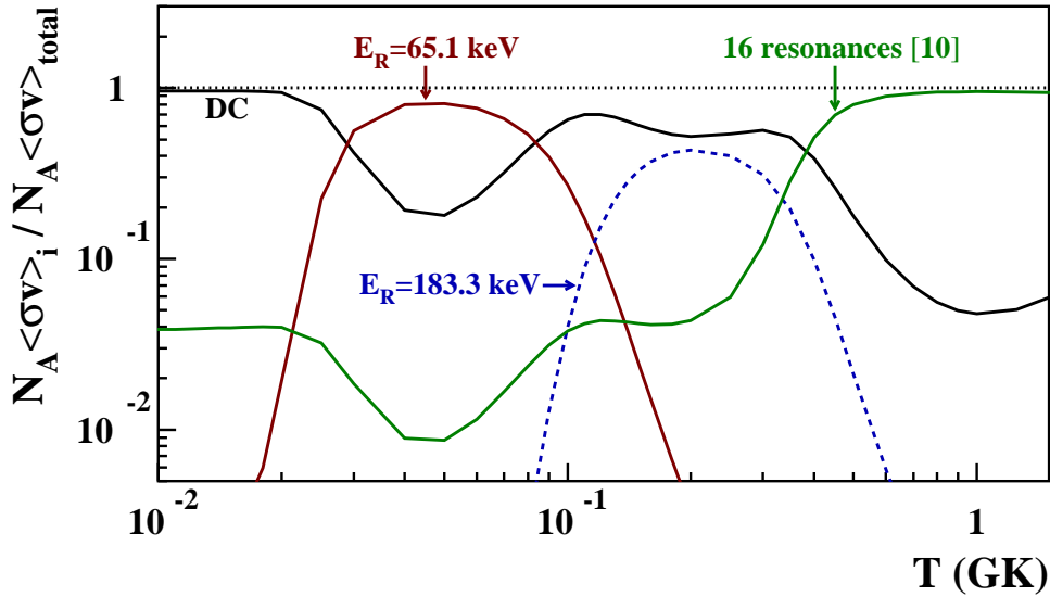
FIG. 11: (Color online) Ratios of individual reaction rate contributions to the total modal rate for the ^{17}\text{O}(p,\gamma)^{18}\text{F} reaction.
