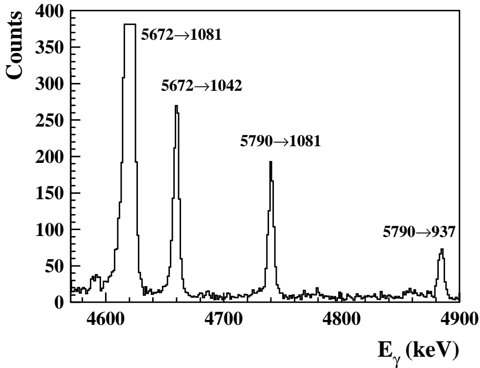
FIG. 2: Relevant section of the \gamma -ray spectrum shown in Fig. 1, taken at \theta_{\text{lab}}=0^{\circ} for E_{\alpha}^{\text{lab}}=1775 keV. The ordinate scale of the figure has been chosen to illustrate the primary \gamma -ray decays of the resonant level at 5790 keV leading to a truncated drawing for the 5672 \rightarrow 1081 keV reference line. The observed weak peak below the 5672 \rightarrow 1081 keV line, identified to the full Doppler-shifted 5603+5605 \rightarrow 0 keV double-escape line, has been included in the least-square fits for energy measurements.
