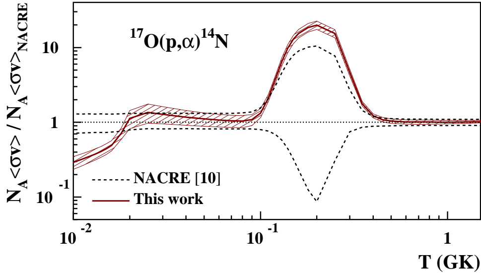
FIG. 9: (Color online) Ratio of present and previous [10] reaction rates for ^{17}\text{O}(p,\alpha)^{14}\text{N} given as the solid line with hatched area representing uncertainties. The dashed lines indicate the previous [10] lower and upper limits for the total rate.
