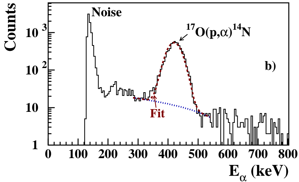
FIG. 4: (Color online) (a) Sample \alpha spectrum obtained in the ^{17}\text{O}(p,\alpha)^{14}\text{N} experiment with the detector at \theta_{\text{lab}}=150^\circ . The proton energy is E_p^{\text{lab}}=196.5 keV and the accumulated charge is equal to 0.93 C. The broad peak labelled ^{11}\text{B}(p,\alpha)^2\text{He} is due to a slight contamination of boron in the used target. (b) Relevant part of the spectrum with a least-squares fit to the data points: dotted line – fitted linear background; dashed line – fitted Gaussian function with intensity, position and standard deviation as free parameters.
