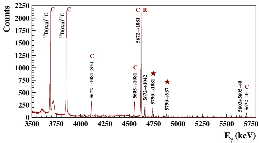
FIG. 1: (Color online) Section of a typical \gamma -ray spectrum obtained at E_{\alpha}^{\text{lab}}=1775 keV with the HPGe detector at \theta_{\text{lab}}=0^{\circ} . The two resonances corresponding to the 5671.6 and 5789.8 keV levels in ^{18}\text{F} were simultaneously populated. A small component due to the weak excitation of the resonant levels at 5603–5605 keV is also visible. The ordinate scale of the figure has been chosen to illustrate some \gamma -ray peaks of relatively low intensities, leading to a truncated drawing for the two lines arising from the ^{10}\text{B}(\alpha,p)^{13}\text{C} reaction. The labels "C" and "R" indicate some of the lines used for calibration and the reference peak for energy difference measurements, respectively (see text). The primary \gamma -ray decays of the resonant level at 5790 keV are labeled with stars. All lines correspond to full-energy peaks unless labeled SE (single-escape line).
