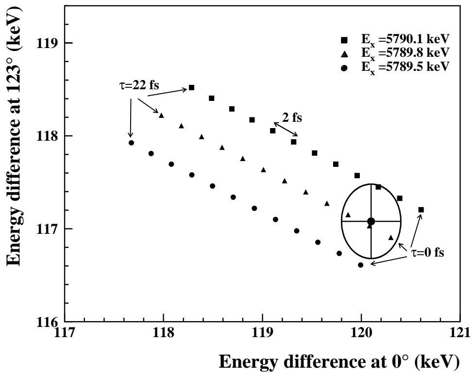
FIG. 3: Calculated and measured values of the differences \Delta_i in the energy of the transitions 5790→1081 keV and 5671.6→1081 keV plotted in the plane \Delta_0 - \Delta_1 (the subscript 0(1) refers to values obtained at 0°(123°)). \Delta_i is calculated for lifetimes of the level at 5790 keV in the range 0–22 fs by a step of 2 fs. The calculated values are given for three different excitation energy values for the level at 5790 keV. As indicated in the text, the lifetime of the 5671.6 keV level is short enough to induce full Doppler shifts of the associated lines. The experimental value is given together with the covariance ellipse corresponding to the bivariate normal distribution of the two independent random variables \Delta_0 and \Delta_1 .
