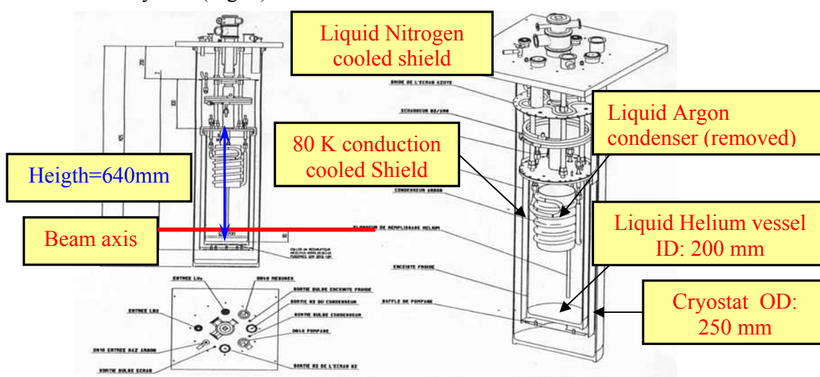
Fig.1: Drawing of the cryostat and the insert
