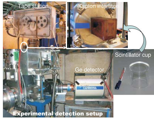
FIG. 2: Detection setup at the end of the PHOENIX Booster beamline. A NE102 scintillator cup surrounds the implantation point for beta counting, and a Germanium detector positioned close to the scintillator provides gamma identification.
