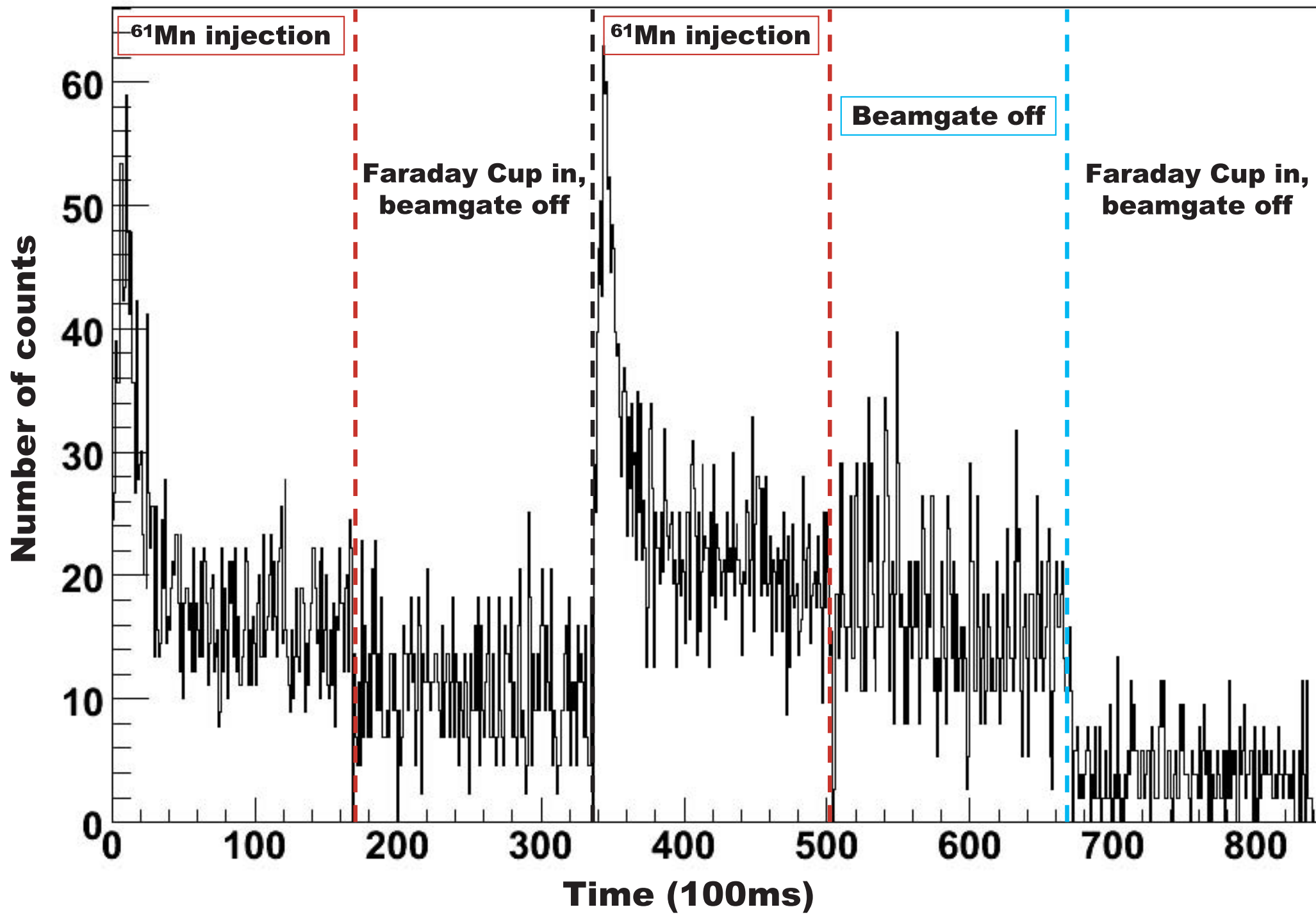
Continuous measurement of ^{61}\text{Fe} decay in various conditions
