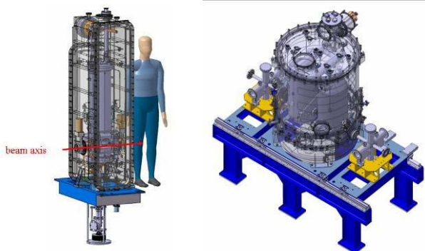
Figure 2: One the 12 cryomodules A and 1 of the 7 cryomodules B.
