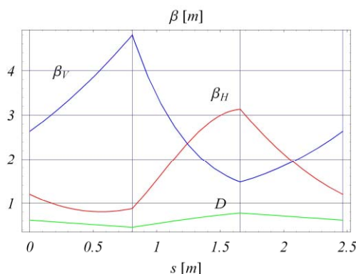
Figure 2: Horizontal and vertical betatron ( \beta_H, \beta_V ) functions and dispersion D in one cell of the spiral FFAG ring.
