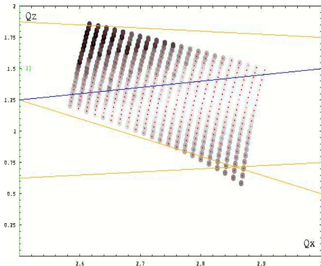
Figure 3: Horizontal dynamical aperture scan in the tune diagram. Points with large dynamical aperture are marked with dark points.
