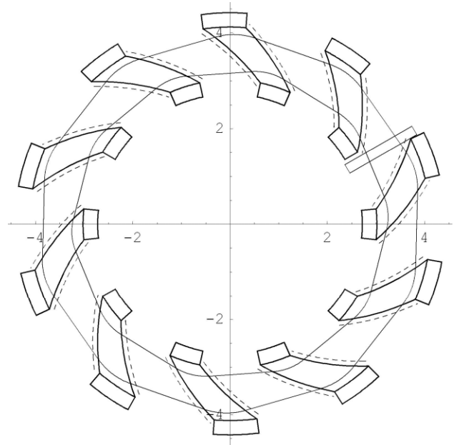
Figure 1: Layout of spiral FFAG for proton therapy. Note the compact size of the ring (dimensions in m).
