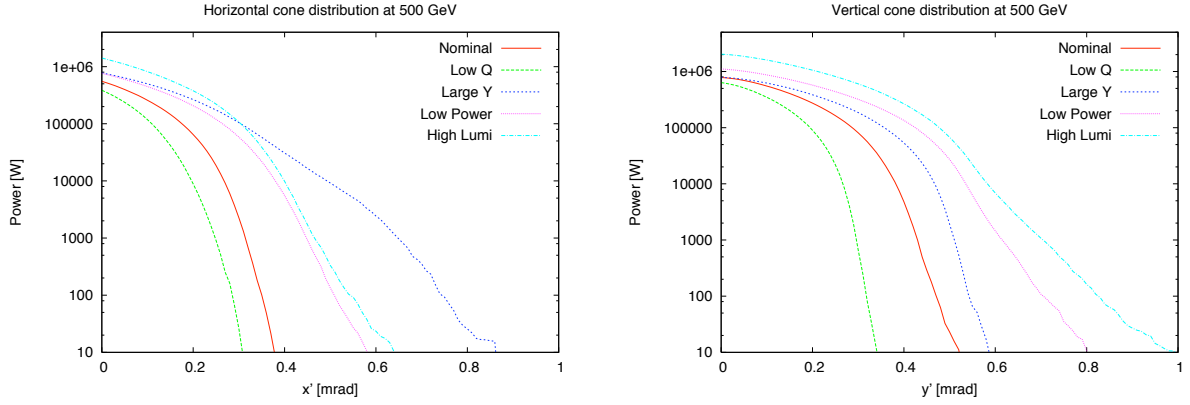
Figure 3: The primary beamstrahlung photon distribution for the 500 GeV machine in the horizontal plane (left) and the vertical plane (right).
