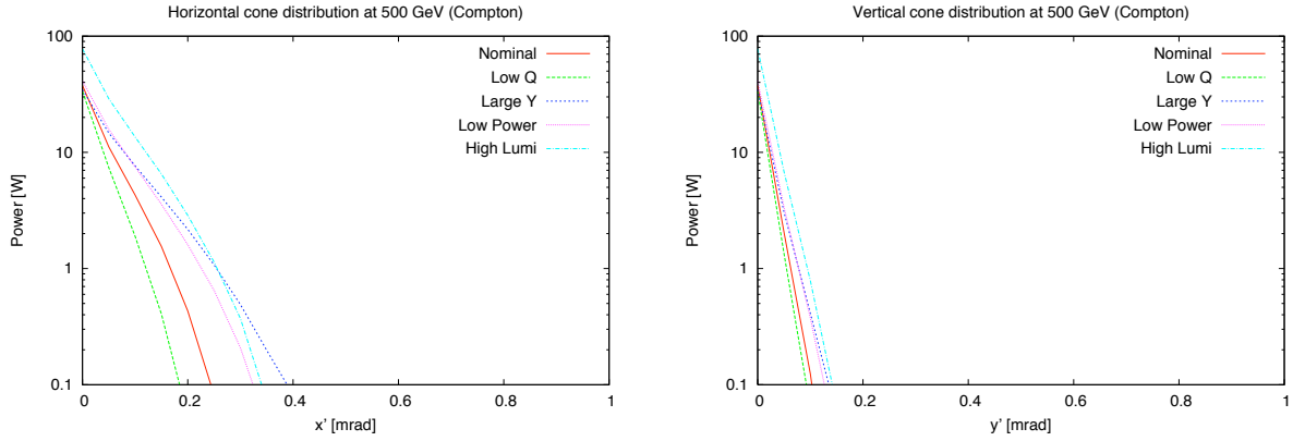
Figure 5: Compton photon distribution for the 500 GeV machine in the horizontal (left) and vertical (right) planes.
