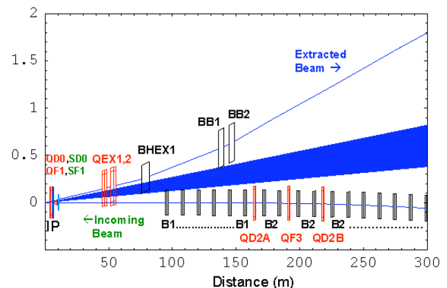
Figure 1: The layout of the minimal 2mrad crossing angle extraction line. The blue cone denotes the photon cone.
