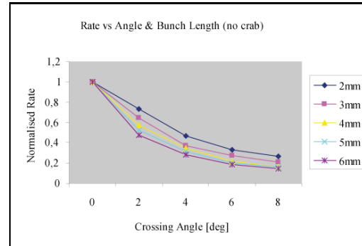
Figure 2: Rate losses as a function of the crossing angle and of the electron bunch length. For 6 mm beams the flux can be reduced also by a factor 5 for a crossing angle of 8 degrees. The laser pulse length is 0.3 mm
