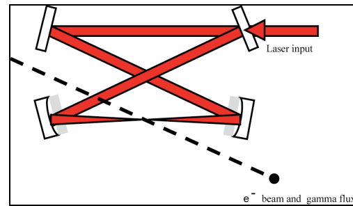
Figure 1: Geometry of the Compton collision for a four mirror optical resonator. The gamma flux will acquire the direction of the colliding electron beam.
