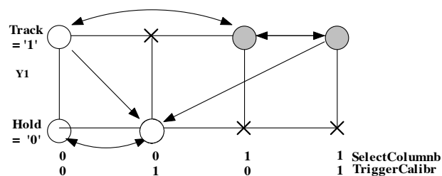
Figure 7: Detailed description of T&H cell
