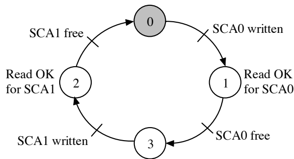
Figure 11: Read operation
