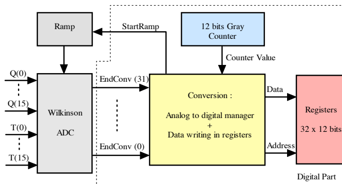
Figure 12: Conversion module
