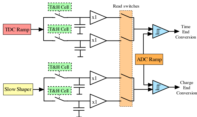
Figure 5: Detail of 1 SCA channel
