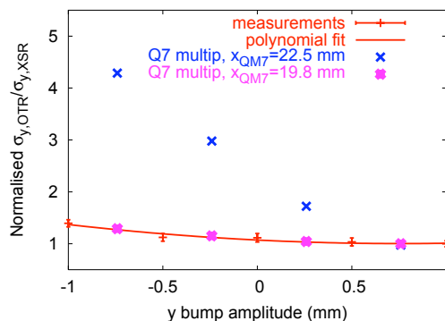
Figure 2: Ratio of the vertical beam sizes at the OTR and at the XSR normalized to the minimum value, measured on the 28 th of May 2008, vs vertical bump amplitude. Results from simulations for two horizontal extraction positions.
