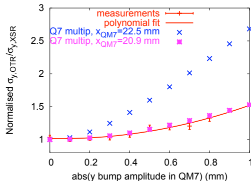
Figure 1: Ratio of the vertical beam sizes at the OTR and at the XSR normalized to the minimum value, measured on the 19 th of December 2007, vs vertical bump amplitude. Results from simulations for two horizontal extraction positions.
