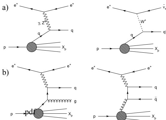
Figure 1: Feynman diagrams indicating LHeC ep ( e -ion) interactions schematically: a) vector boson ( \gamma, Z^0, W^\pm ) exchange within the framework of SM eq \rightarrow eq and eq \rightarrow \nu q (“neutral and charged current”) scattering; the interacting q momentum is specified by the “parton density function” (pdf) of the incoming proton; b) a q in the dense QCD field of the p (ion), which has evolved chromodynamically ( g radiation), interacting with the e .
