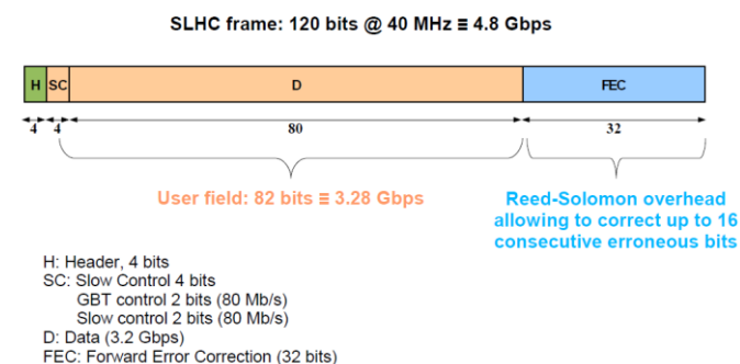
Figure 3: GBT frame
