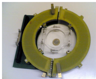
Figure 3: Triple-GEM ring detectors, composing one of the two trackers installed on each side of the IR.
