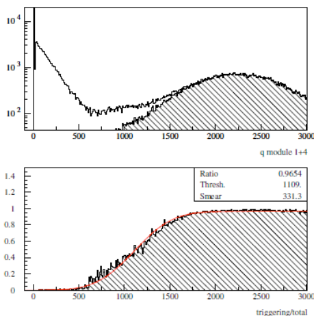
Figure 4: Determination of the trigger threshold by taking the ratio of triggering/total events in one module.
