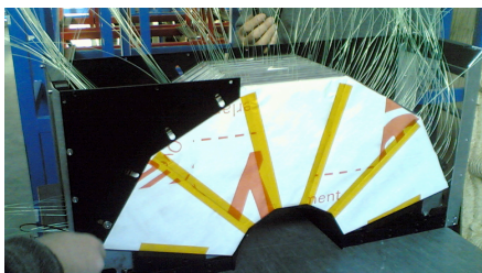
Figure 2: One of the four Bhabha calorimeter modules, each composed by five sectors of 12 scintillator trapezoidal tiles sandwiching 11 lead plates.
