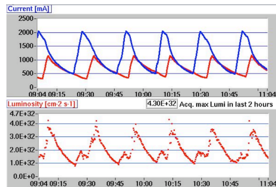
Figure 5: Online display of the currents in the machine (upper plot) and the luminosity measured by our luminometers (bottom plot, including the correction for the acceptance and background subtraction).
