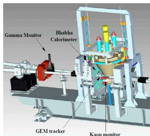
Figure 1: View of the DAFNE interaction region, with the detectors for luminosity measurement around the SIDDHARTA experiment setup.
