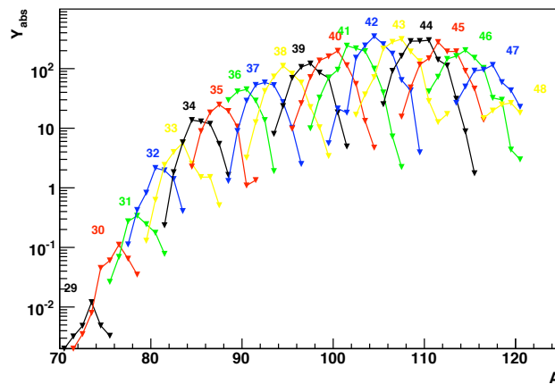
Figure 17: Absolute isotopic yields of thermal-neutron induced fission of ^{249}\text{Cf} . The corresponding fission-fragment atomic numbers are indicated.
