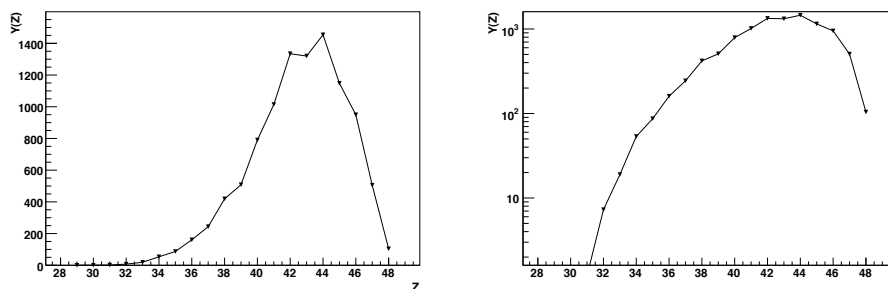
Figure 18: Element yields of thermal-neutron induced fission of ^{249}\text{Cf} , in linear and logarithmic scale.
