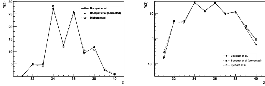
Figure 3: Absolute element yields of thermal-neutron induced fission of ^{229}\text{Th} .
