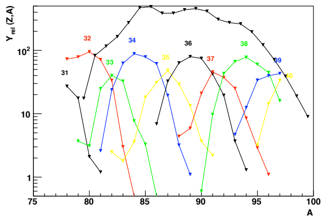
Figure 1: Relative isotopic yields of thermal-neutron induced fission of ^{229}\text{Th} . The corresponding fission-fragment atomic numbers are indicated. The mass yields multiplied by a factor 50 are displayed for comparison.
