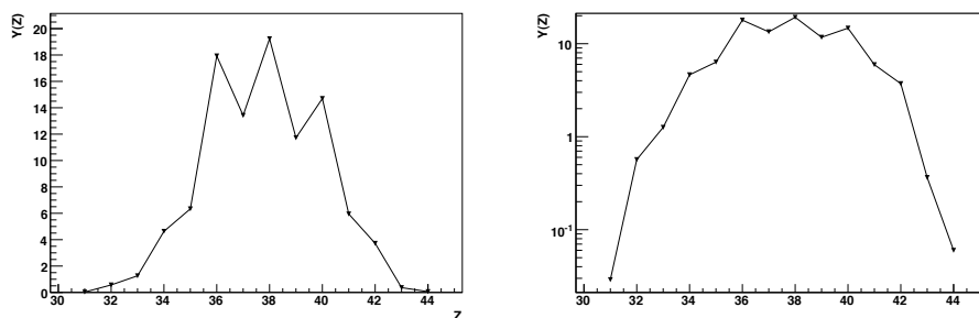
Figure 10: Element yields of thermal-neutron induced fission of ^{233}\text{U} , in linear and logarithmic scale.
