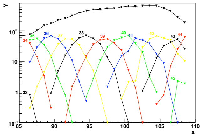
Figure 11: Isotopic yields of thermal-neutron induced fission of ^{239}\text{Pu} . The corresponding fission-fragment atomic numbers are indicated. The mass yield is represented on the same Figure, multiplied by a factor 100.
