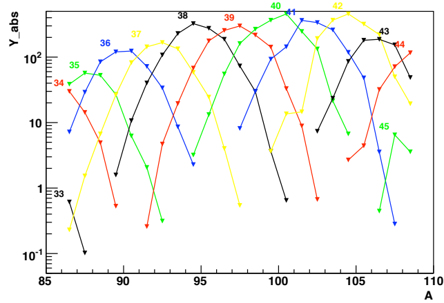
Figure 12: Isotopic yields of thermal-neutron induced fission of ^{239}\text{Pu} . The corresponding fission-fragment atomic numbers are indicated.
