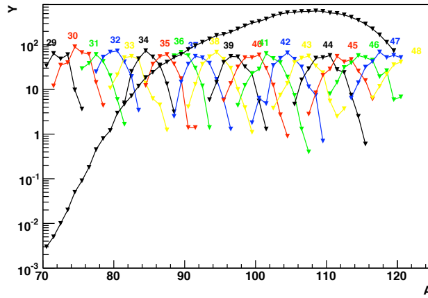
Figure 16: Isotopic yields of thermal-neutron induced fission of ^{249}\text{Cf} . The corresponding fission-fragment atomic numbers are indicated. The mass yield is represented on the same Figure, multiplied by a factor 100 for clarity.
