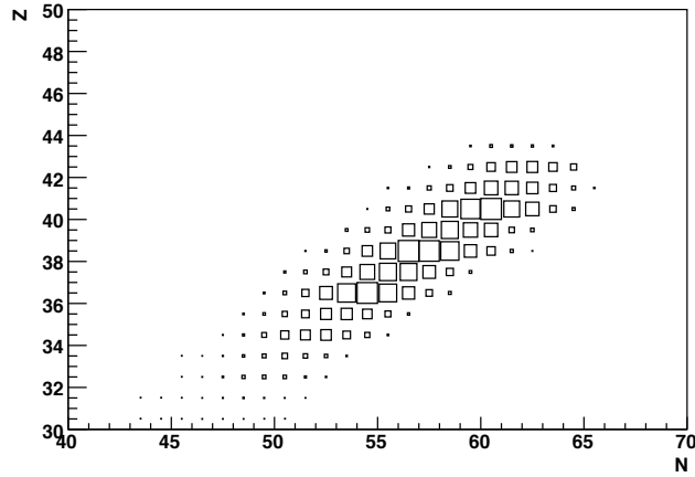
Figure 8: Isotopic yields of thermal-neutron induced fission of ^{235}\text{U} , in a 2-dimensional nuclide chart.
