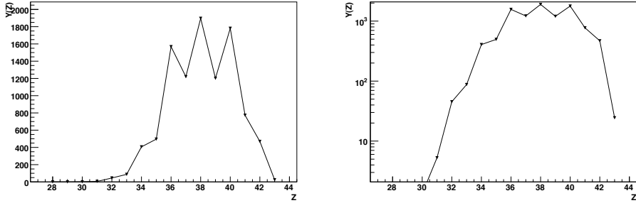
Figure 7: Element yields of thermal-neutron induced fission of ^{235}\text{U} , in linear and logarithmic scale.
