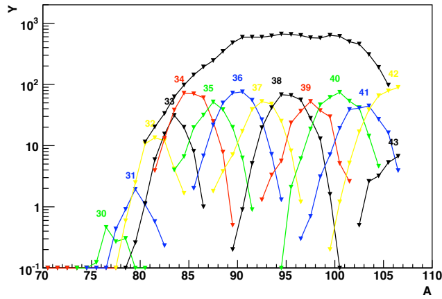
Figure 4: Isotopic yields of thermal-neutron induced fission of ^{235}\text{U} . The corresponding fission-fragment atomic numbers are displayed. The mass yields multiplied by a factor of 100 are displayed.
