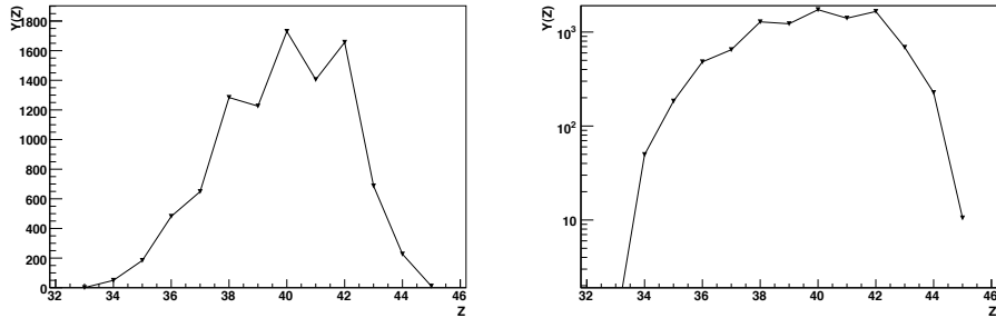
Figure 13: Element yields of thermal-neutron induced fission of ^{239}\text{Pu} , in linear and logarithmic scale.
