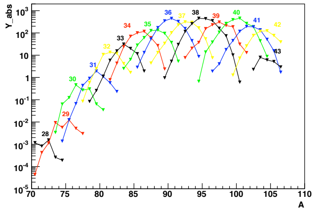
Figure 6: Absolute isotopic yields of thermal-neutron induced fission of ^{235}\text{U} . The corresponding fission-fragment atomic numbers are displayed.
