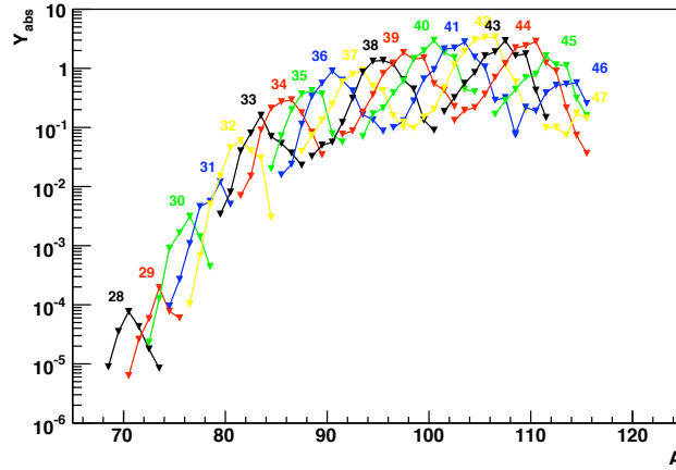
Figure 14: Absolute isotopic yields of thermal-neutron induced fission of ^{245}\text{Cm} . The corresponding fission-fragment atomic numbers are displayed.
