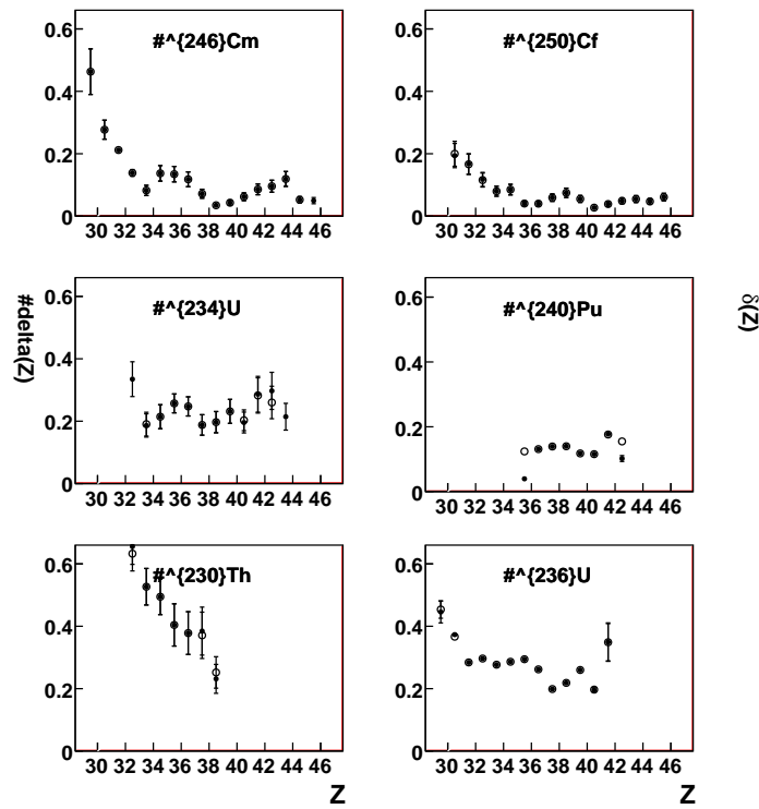
Figure 19: Local even-odd effect for the different systems studied at Lohengrin (full circles). When truncated and if possible, the isotopic distributions are completed by gaussian extrapolation. The resulting even-odd effect is displayed with open circles.
