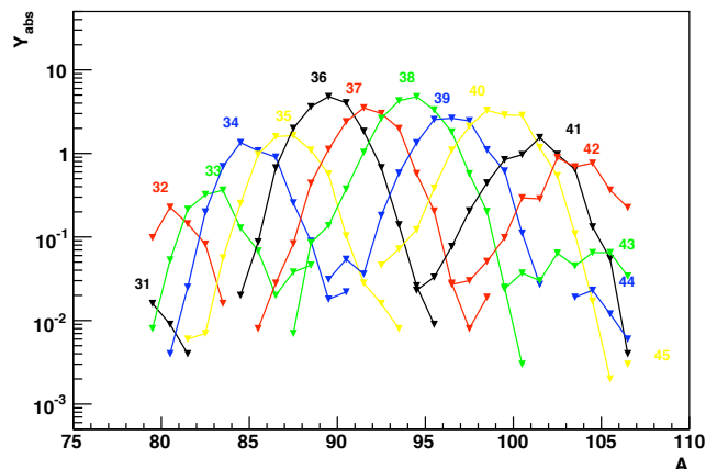
Figure 9: Absolute isotopic yields of thermal-neutron induced fission of ^{233}\text{U} . The corresponding fission-fragment atomic numbers are displayed.
