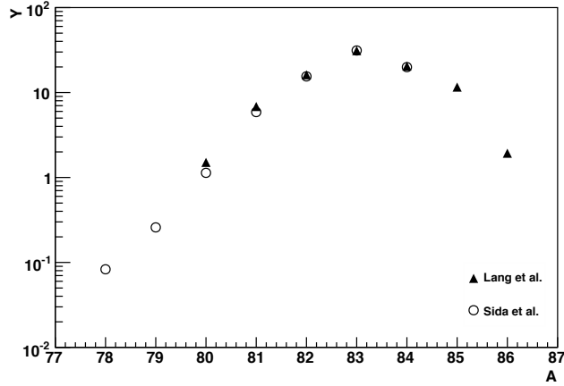
Figure 5: Absolute isotopic yields of Z=33 in thermal-neutron induced fission of ^{235}\text{U} , as given in references [3] and [4] with full triangles and open circles, respectively.
