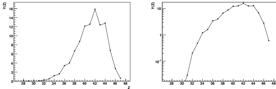
Figure 15: Element yields of thermal-neutron induced fission of ^{245}\text{Cm} , in linear and logarithmic scale.
