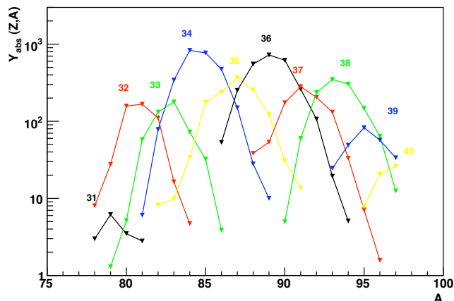
Figure 2: Absolute isotopic yields of thermal-neutron induced fission of ^{229}\text{Th} . The corresponding fission-fragment atomic numbers are indicated.
