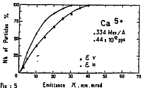
Fig : 5 Emittance X , mm.mrad
