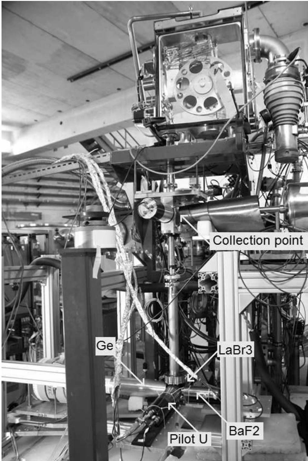
Figure 1: The experimental setup used at ALTO for the fast-timing measurements.
