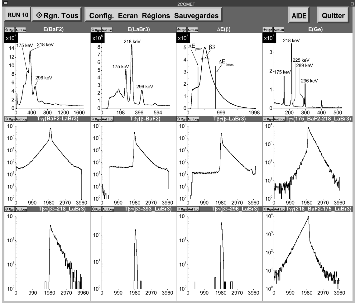
Figure 2: On-line screen capture of the NARVAL acquisition spectrum window. The energy (or \Delta E for \beta detector) singles spectra are shown on the first row. The first three spectra displayed on the second row are the TAC singles spectra; they are marked by the name of the detectors used as start and stop signals. The other spectra are double-gated TAC spectra, they are labeled by the energy conditions required to accept the start and stop signals.
