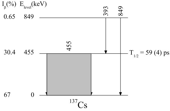
Figure 6: Partial level scheme of ^{137}\text{Cs} obtained from the decay of ^{137}\text{Xe} ; the arrow width is proportional to the \gamma intensity of the transitions; data are taken from ref. [13], except the half-life (this work).
