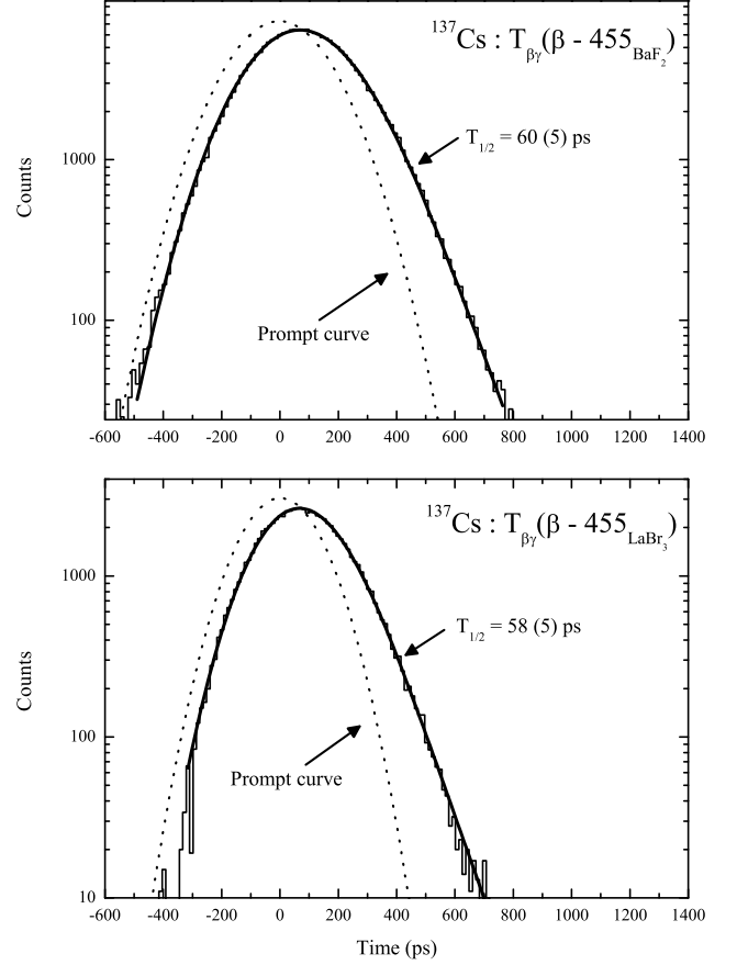
Figure 8: Time spectra for the determination of the half-life of the 455.5 keV state in ^{137}\text{Cs} ; the solid line represents the best fit of the data, the half-life arising from the best fit is indicated.
