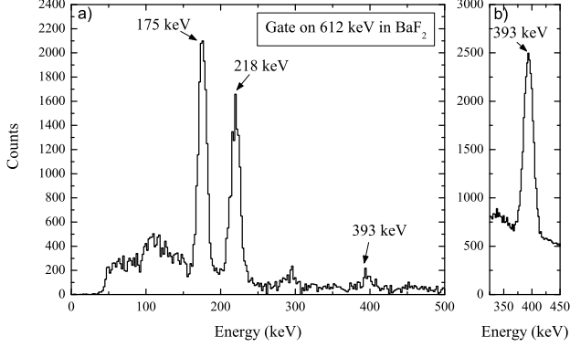
Figure 12: a) \text{LaBr}_3 projection spectrum extracted from the \mathcal{M}(E_{\text{BaF}_2} - E_{\text{LaBr}_3} - T_{\text{BaF}_2 - \text{LaBr}_3}) matrix by gating the \text{BaF}_2 detector on the 612 keV \gamma line. b) Partial \text{LaBr}_3 projection spectrum extracted from the \mathcal{M}(E_{\beta} - E_{\text{LaBr}_3} - T_{\beta - \text{LaBr}_3}) matrix by setting on the \beta detector the gate defined by \Delta E_{\beta \min} and \Delta E_{\beta \max} .
