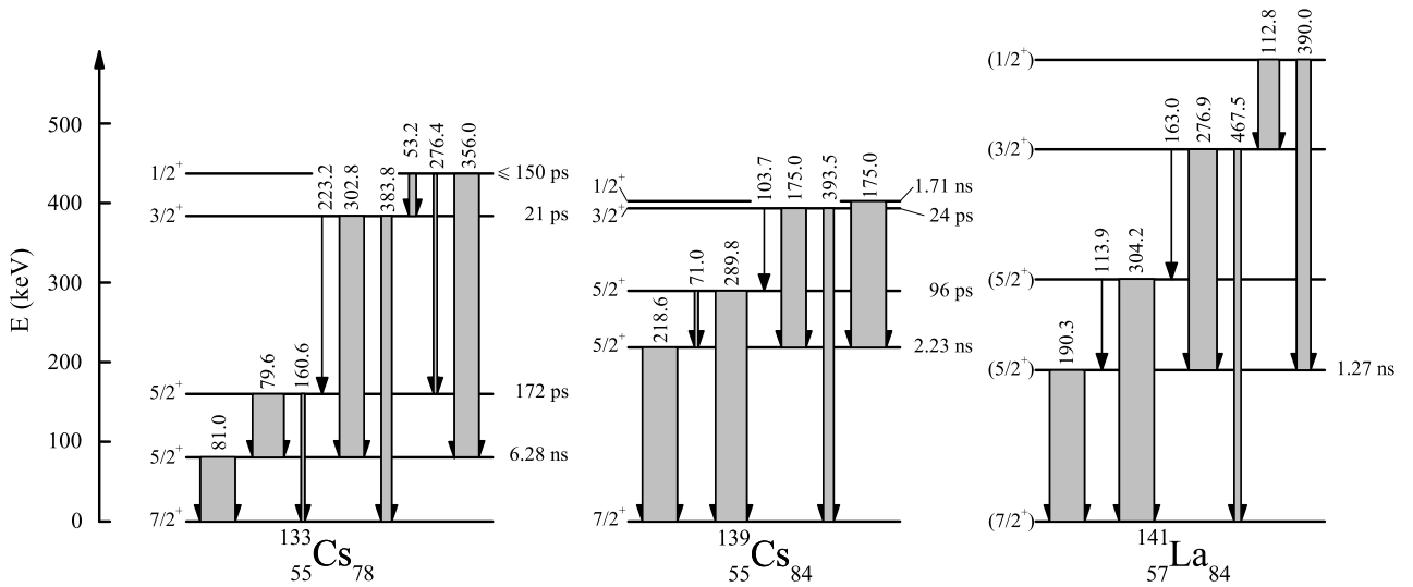
Figure 15: Comparison between the first four excited levels in ^{133,139}\text{Cs} and ^{141}\text{La} . The experimental data were taken from this work and refs. [15, 27, 29]. The transition energies are indicated in keV. The arrow width is proportional to the total intensity of the transitions. For each level, the sum of the total intensities of the transitions has been normalized to 100.
