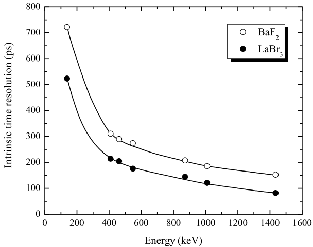
Figure 3: Intrinsic time resolution of the BaF 2 and LaBr 3 detectors.
