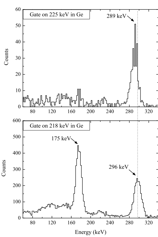
Figure 10: \text{LaBr}_3 projection spectra extracted from the \mathcal{M}(E_{\text{LaBr}_3} - E_{\text{Ge}} - T_{\beta\text{-LaBr}_3}) matrix by gating the Ge(HP) detector on the 218 and 225 keV \gamma rays.
