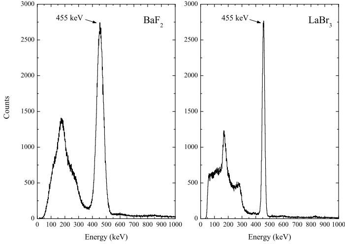
Figure 7: \text{BaF}_2 and \text{LaBr}_3 projection spectra extracted from the \mathcal{M}(E_{\beta}-E_{\text{BaF}_2}-T_{\beta-\text{BaF}_2}) and \mathcal{M}(E_{\beta}-E_{\text{LaBr}_3}-T_{\beta-\text{LaBr}_3}) matrices by setting a gate defined by \Delta E_{\beta\text{min}} and \Delta E_{\beta\text{max}} (see sect. 2) on the \beta detector.
