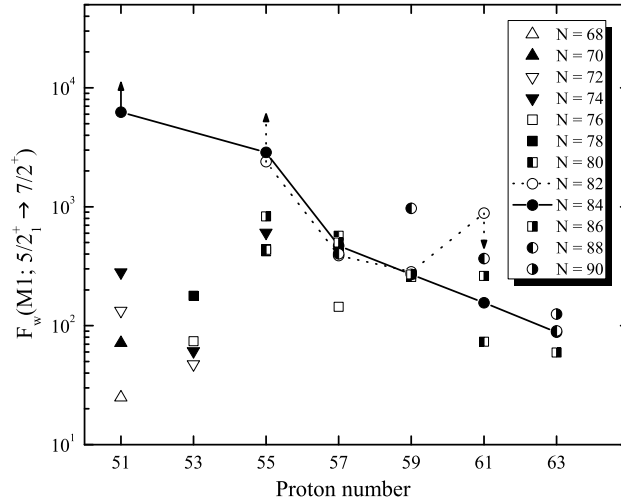
Figure 14: Weisskopf M1 hindrance factors for the \frac{5}{2}_1^+ \rightarrow \frac{7}{2}_1^+ transitions known in the Sb to Eu isotopes. Data are taken from refs. [13, 15, 20-35]. When the \frac{5}{2}_1^+ state is the ground state, the experimental B(M1) used to calculate the hindrance factor was modified by the \frac{8}{6} factor corresponding to (2I_i+1)/(2I_f+1) .
