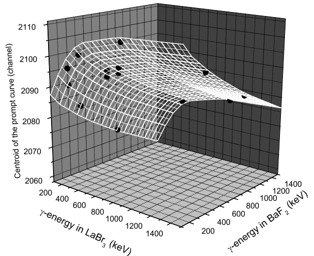
Figure 4: Centroids of the prompt curve for time measurements performed between the BaF 2 and LaBr 3 detectors. The dots represent the measured values and the grid the values determined from the \beta -BaF 2 and \beta -LaBr 3 time measurements on the A = 138 mass.
