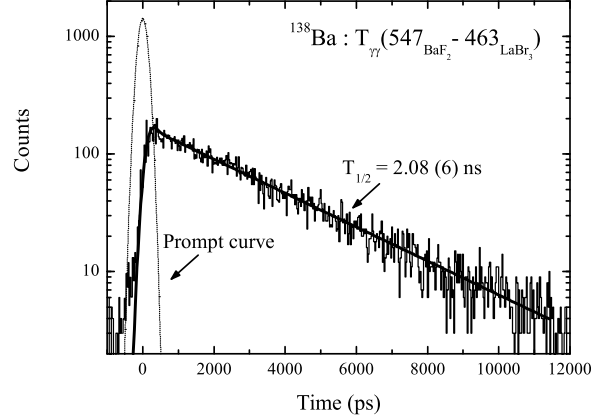
Figure 5: Partial level scheme of ^{138}\text{Ba} obtained from the decay of ^{138}\text{Cs} ; the arrow widths are proportional to the \gamma intensity of the transitions; more than 90 % of the decay intensity is displayed; data are taken from ref. [11]. Three time spectra for the half-life determination of the 1899 keV level of ^{138}\text{Ba} ; the solid line represents the best fit of the data, the half-life arising from the best fit is indicated.
