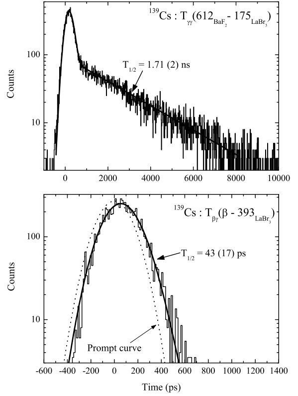
Figure 13: Time spectra for the half-life determination of excited levels in ^{139}\text{Cs} . The upper spectrum shows two components due to the half-lives of the 393 and 394 keV levels, the lower spectrum gives access to T_{1/2}(393 \text{ keV}) .
