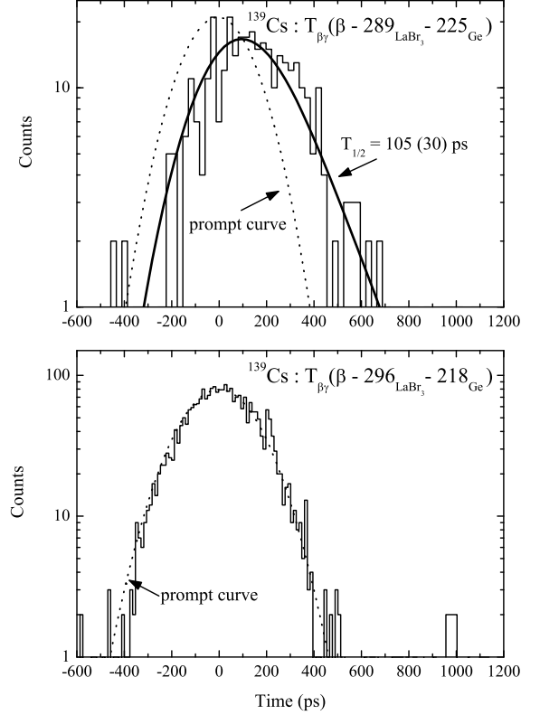
Figure 11: Time spectra for the half-life determination of levels in ^{139}\text{Cs} . The upper spectrum gives access to T_{1/2}(515 \text{ keV}) + T_{1/2}(289 \text{ keV}) , the lower spectrum to T_{1/2}(515 \text{ keV}) .
