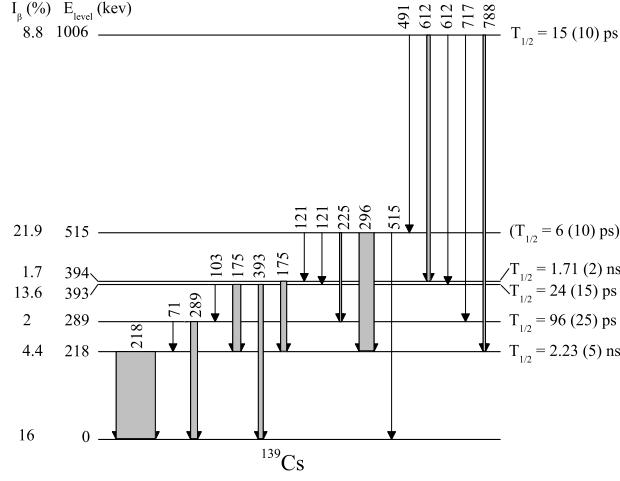
Figure 9: Partial level scheme of ^{139}\text{Cs} obtained from the decay of ^{139}\text{Xe} ; the arrow width is proportional to the \gamma intensity of the transitions; data are taken from ref. [15], except the half-lives (this work).
