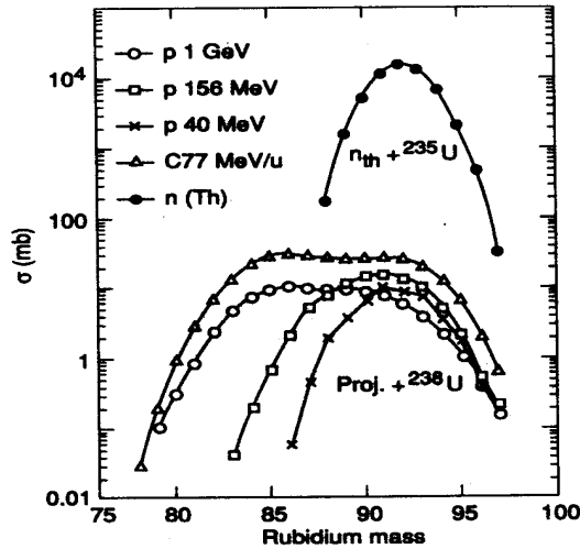
Fig 1. Production cross section of Rubidium isotopes
