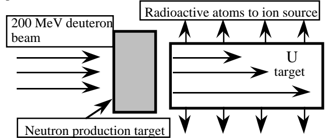
Fig. 3. Second generation targets principle
