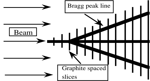
Fig 2. Conical graphite target proposed at SPIRAL.
